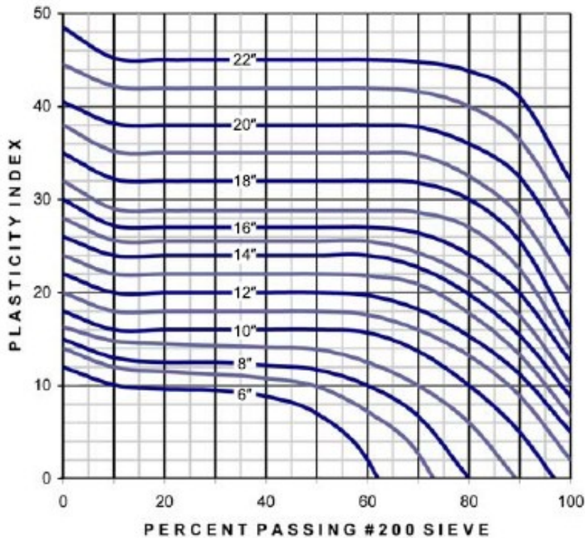
FIGURE 5-10.3 BASE COURSE FOR LOCAL AND MINOR COLLECTORS, LOCAL COMMERCIAL AND LOCAL INDUSTRIAL STREETS
