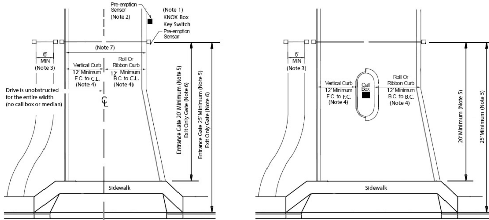
A. Unobstructed Gated Driveway Entrance or Exit with Emergency or Service Vehicle Access Through Gated Entrance or Exit.
