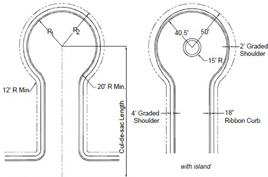
FIGURE 5-3.44 CUL-DE-SAC STREET LENGTH
