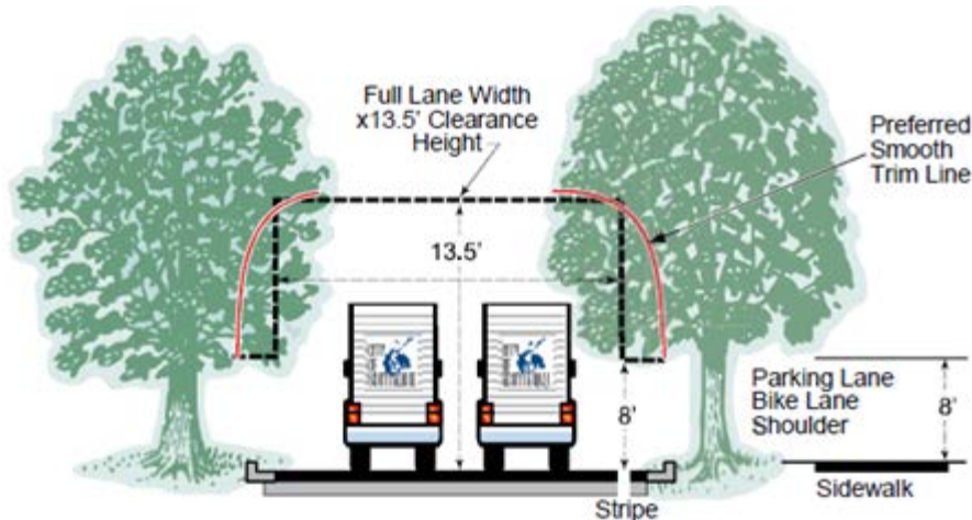
FIGURE 8-1.3 ARTERIAL OR COLLECTOR ROADWAY CLEARANCES (35 MILES PER HOUR (MPH) OR GREATER) LANDSCAPED MEDIANS/ROWS
