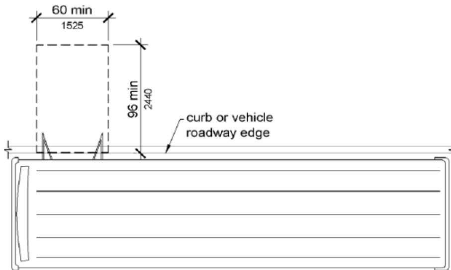
FIGURE 5-6.4 BUS STOP CLEARANCE ZONES
