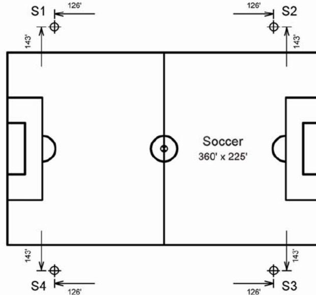
FIGURE 8-2.2 SOCCER POLE LOCATIONS
