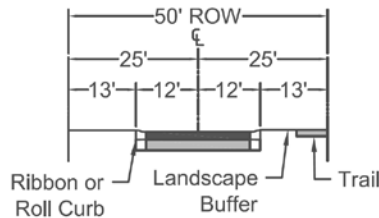
FIGURE 5-3.18 LOCAL RESIDENTIAL -- RURAL/ESL WITH TRAILS
