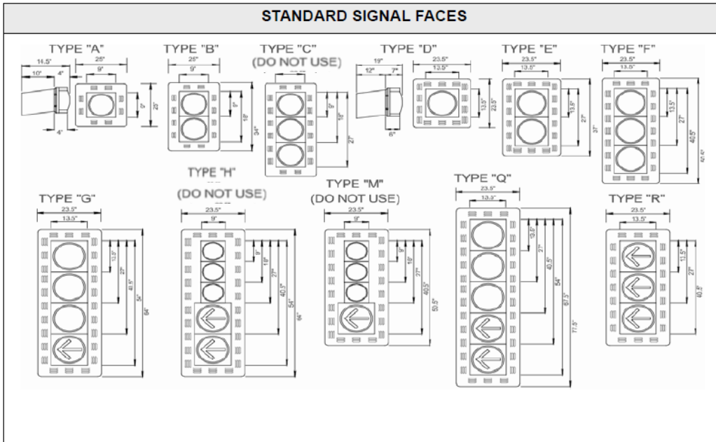
FIGURE 5-4.1 STANDARD SIGNAL FACES
