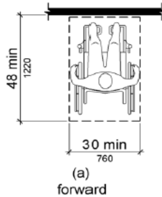
FIGURE 5-6.5 BUS SHELTER CLEARANCE ZONES
