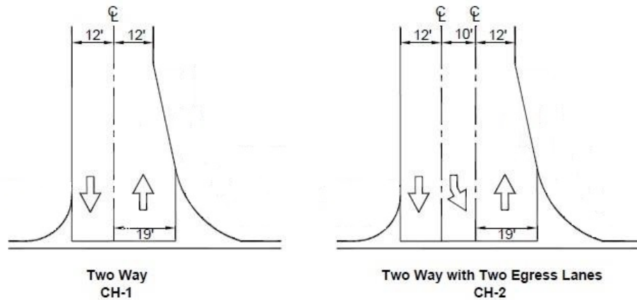
FIGURE 5-3.38 TYPE CH TWO-WAY DRIVEWAYS
