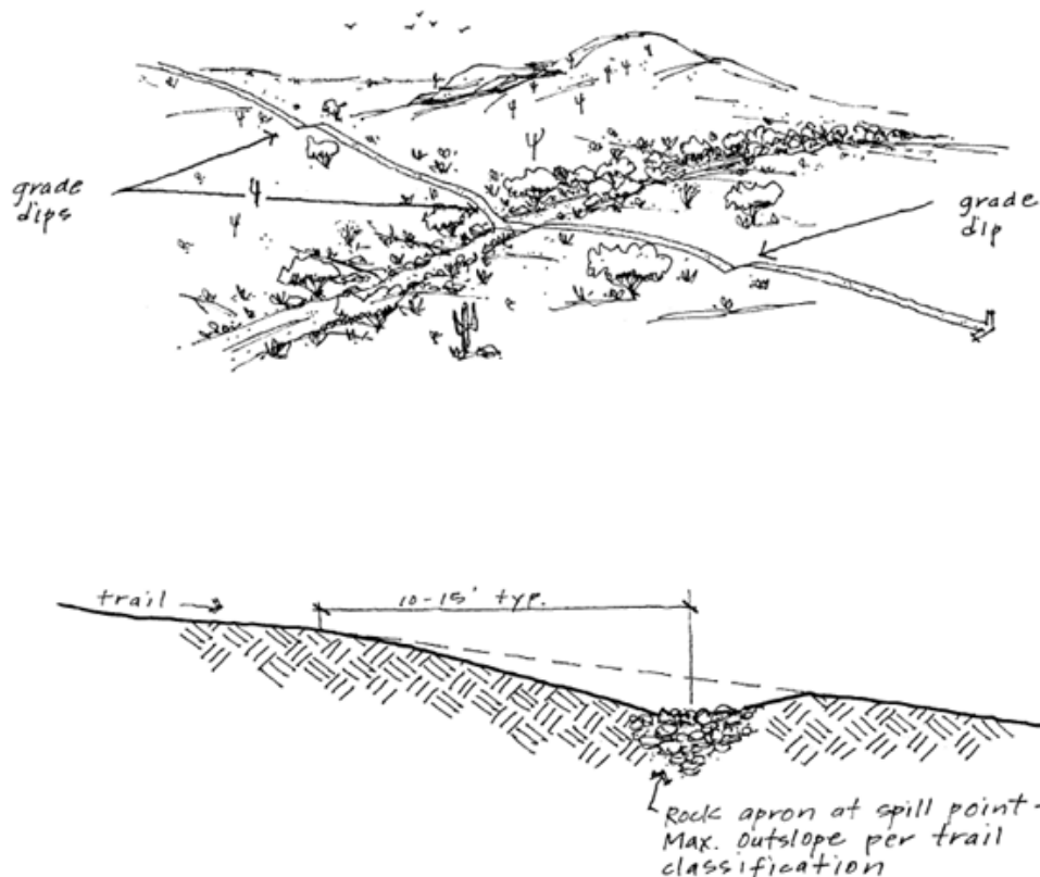
FIGURE 8-3.5 GRADE DIPS
