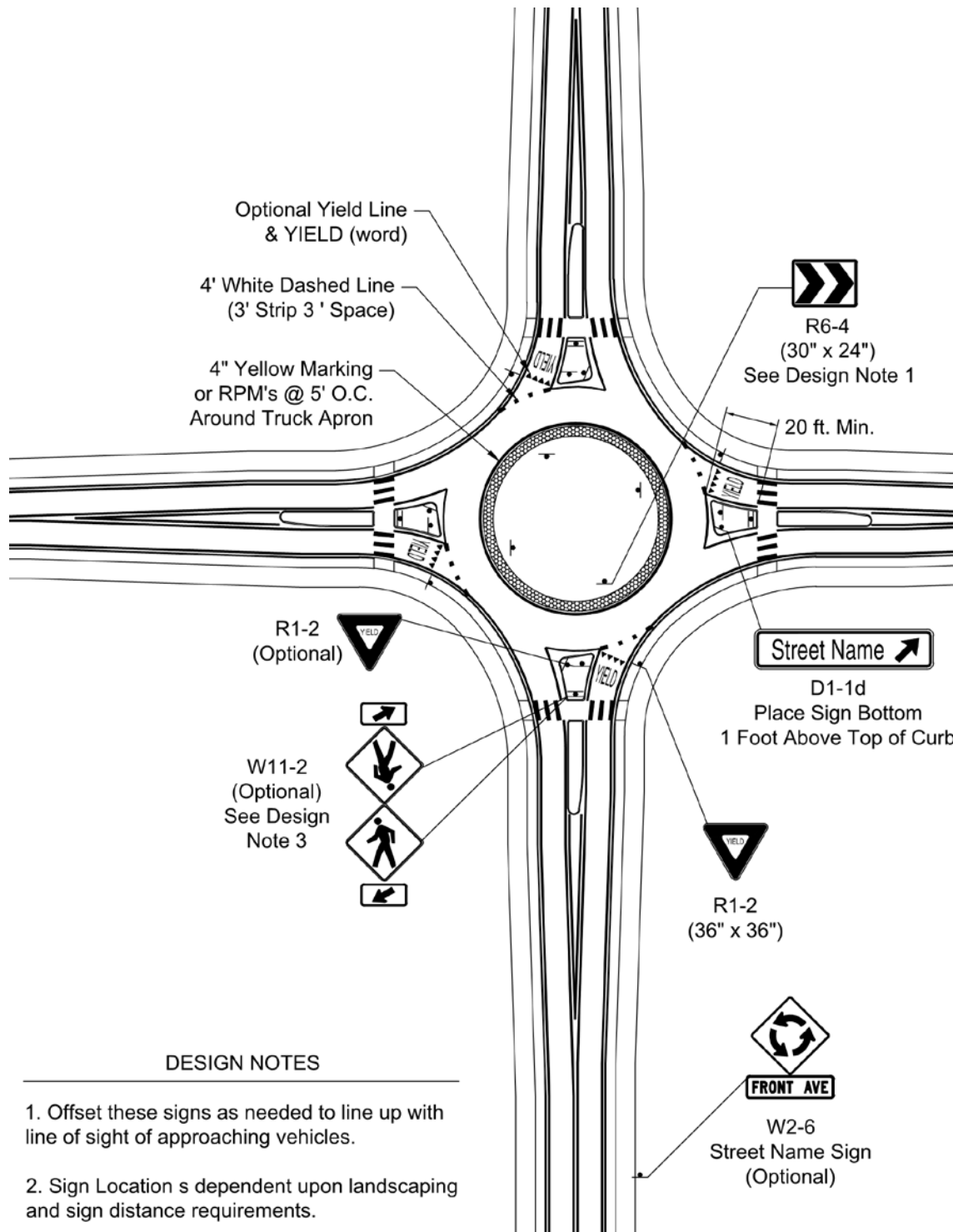
FIGURE 5-3.33 ROUNDABOUT SIGNING AND MARKINGS
