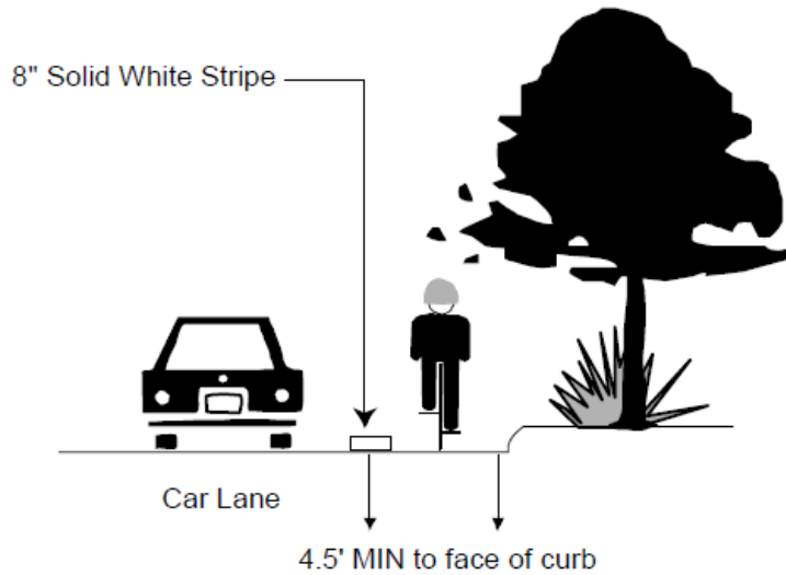
FIGURE 5-7.2 BIKE LANE WITH WIDE CURB LANES
