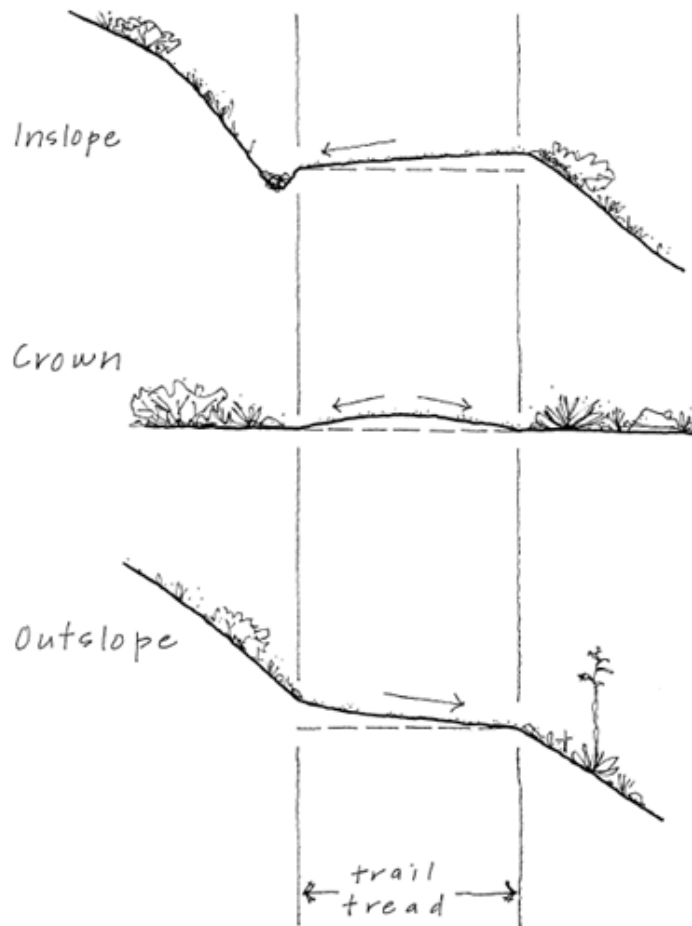
FIGURE 8-3.1 CROSS SLOPES
