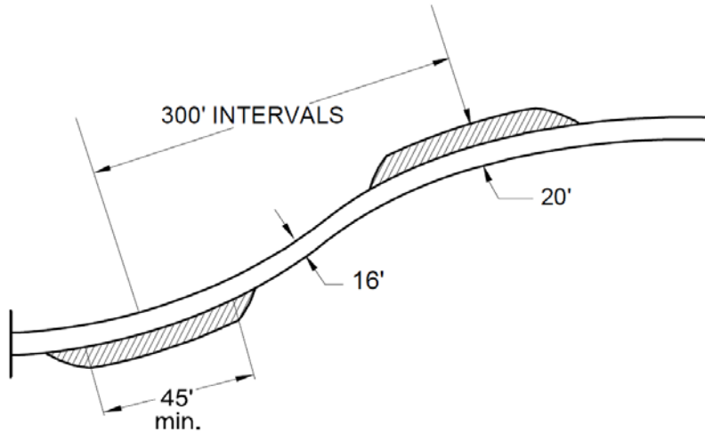
FIGURE 2-2.6 FIRE TURN-OUT FOR EXTENDED DRIVEWAYS
