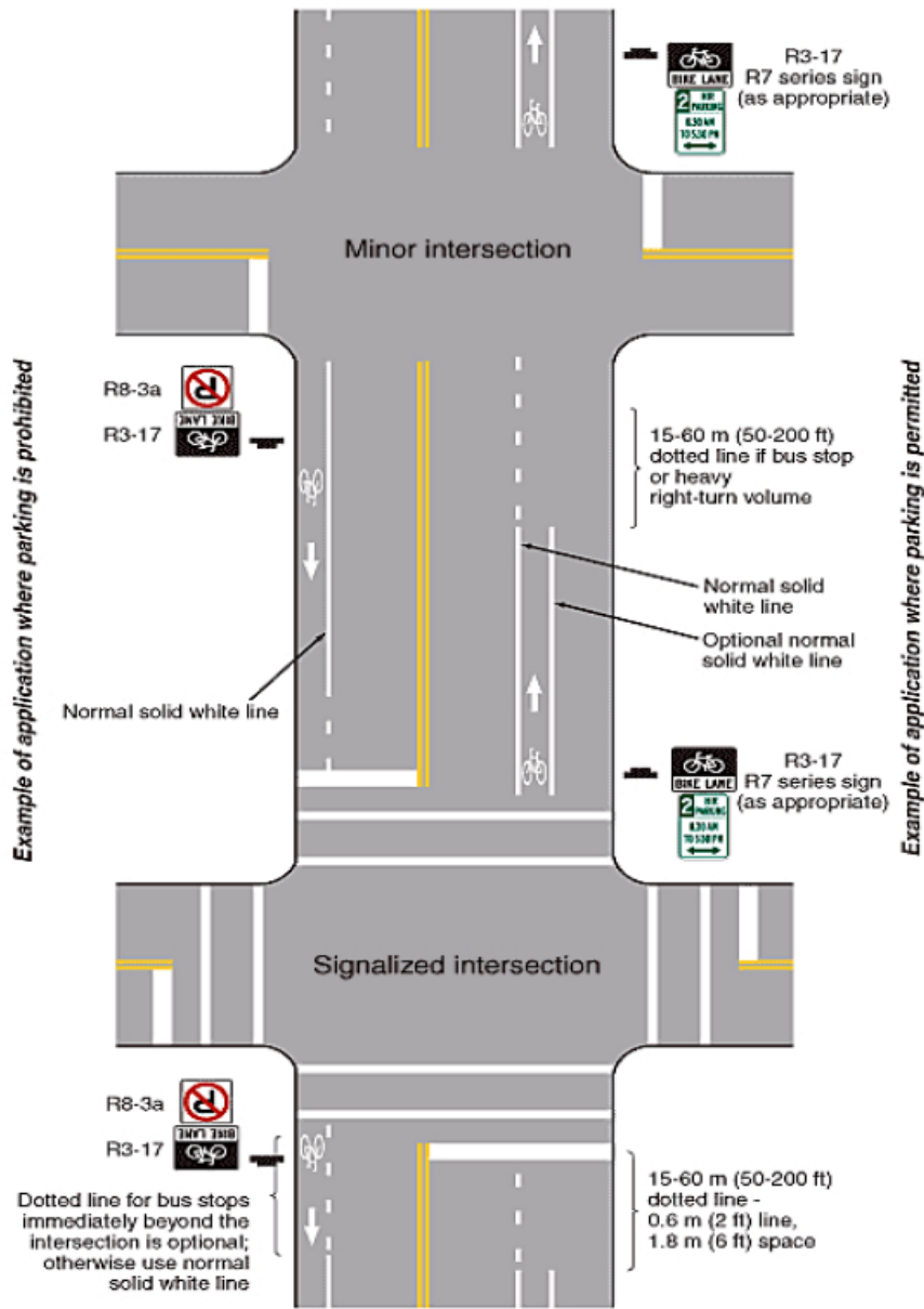
FIGURE 5-7.15 EXAMPLES OF PAVEMENT MARKINGS FOR BICYCLE LANES ON A TWO-WAY STREET; AND
