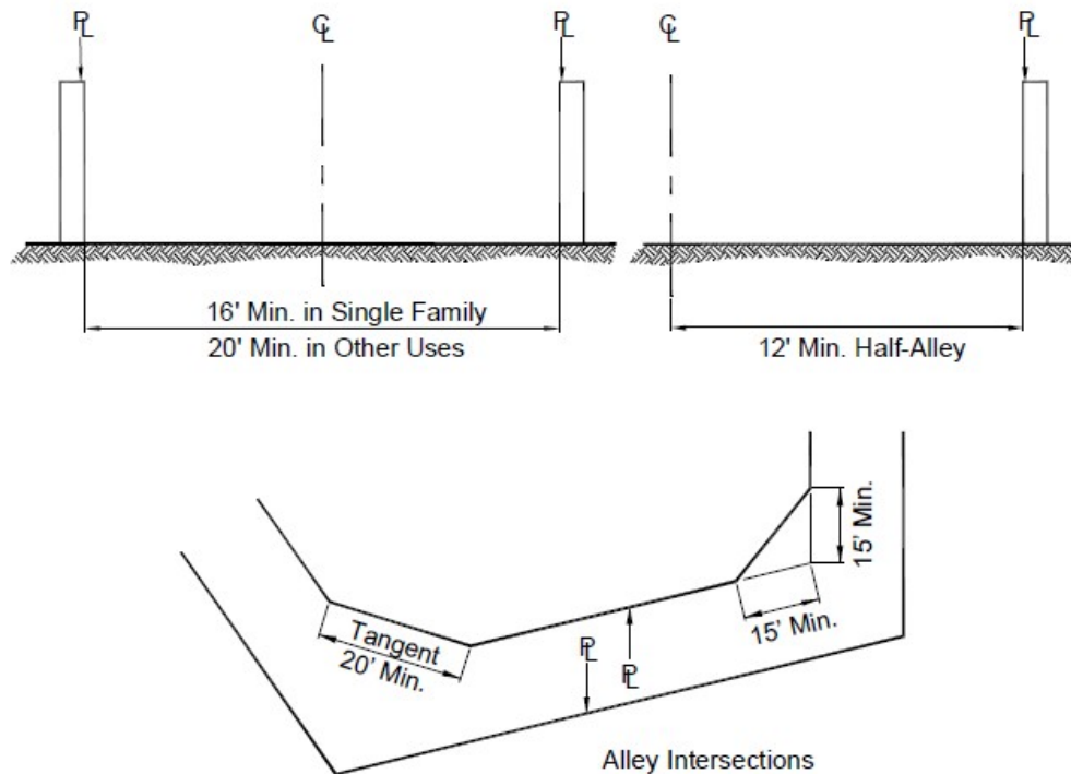
FIGURE 5-3.46 ALLEY WIDTHS AND INTERSECTIONS
