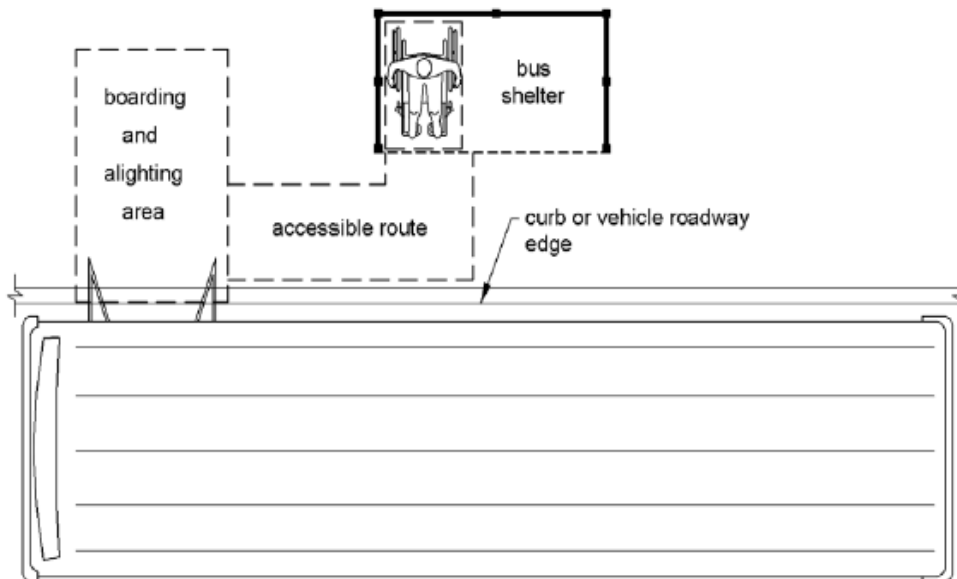
FIGURE 5-6.6 BUS SHELTER BOARDING AND ALIGHTING AREA
