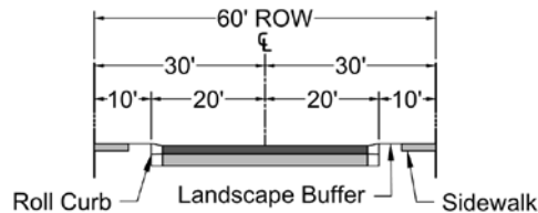
FIGURE 5-3.21 LOCAL COMMERCIAL/INDUSTRIAL
