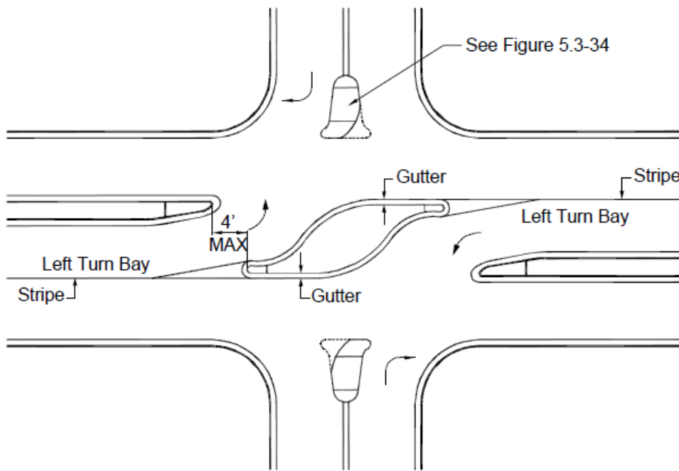
FIGURE 5-3.30 LEFT IN / LEFT IN MEDIAN OPENINGS FOR INTERSECTIONS
