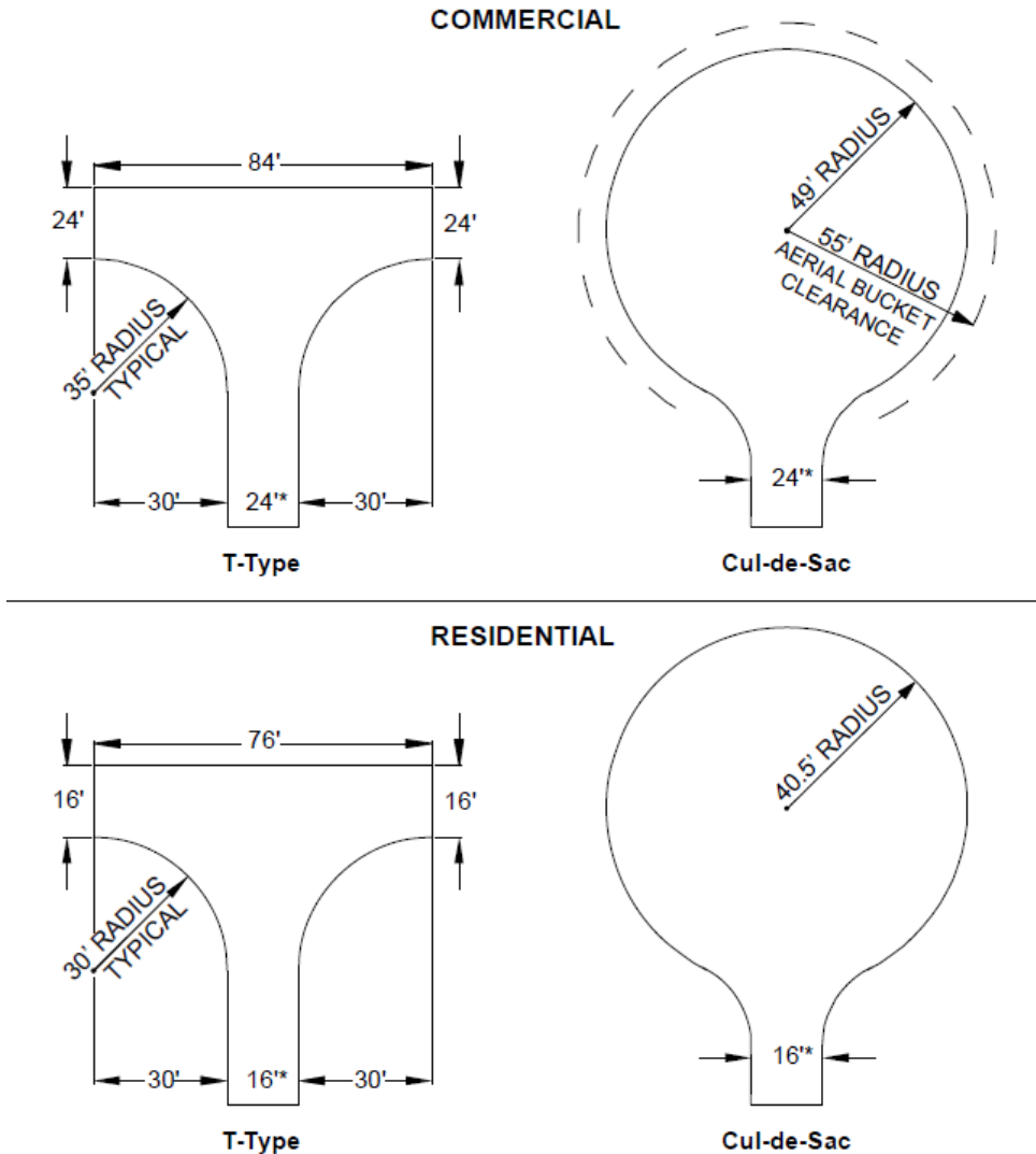
FIGURE 2-1.5 FIRE LANE FIRE ACCESS TURNAROUNDS
