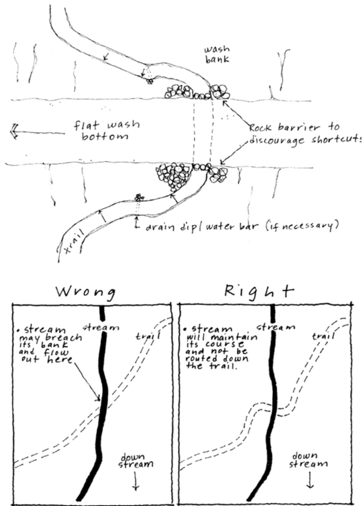
FIGURE 8-3.12 DESERT WASH CROSSING
