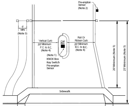
C. Obstructed Gated Driveway Entrance with Emergency or Service Vehicle Access Through Gated Entrance.
