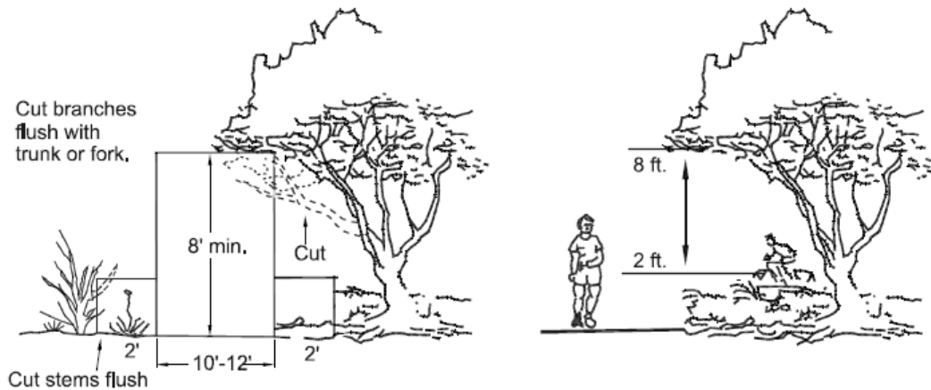
FIGURE 5-7.9 PATH VEGETATION CLEARANCE
