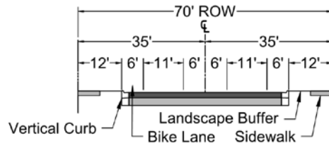
FIGURE 5-3.14 MINOR COLLECTORS -- URBAN CHARACTER
