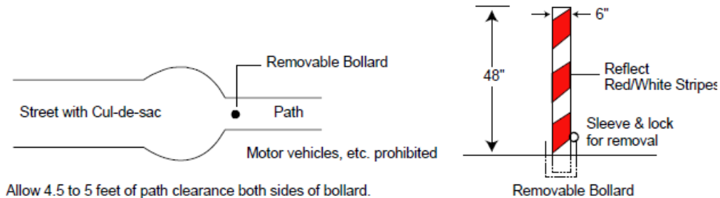
FIGURE 5-7.14 VEHICLE CONTROL PATH ENTRANCE (WHERE NEEDED)
