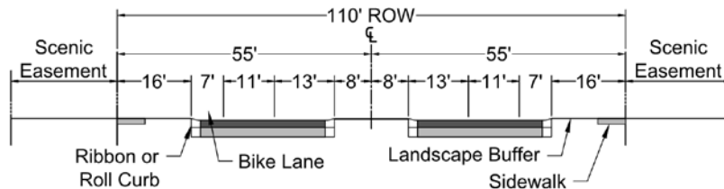
FIGURE 5-3.4 MINOR ARTERIALS -- RURAL/ESL CHARACTER
