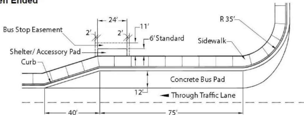
FIGURE 5-6.11 BUS BAYS
