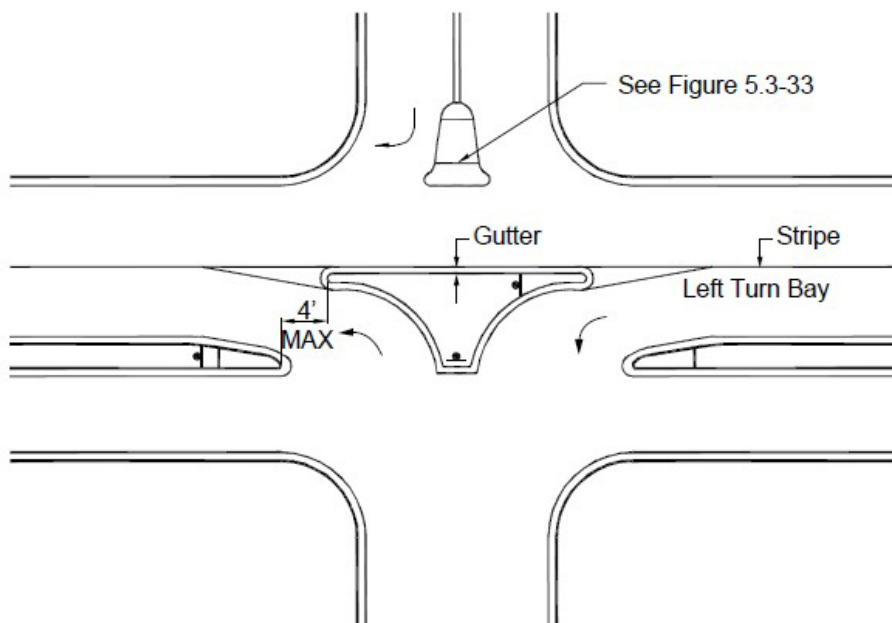
FIGURE 5-3.28 MEDIAN OPENINGS FOR INTERSECTIONS
