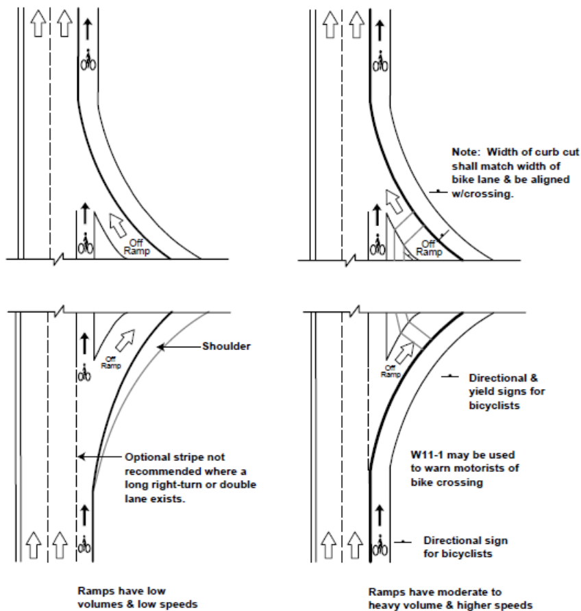
FIGURE 5-7.13 RAMP CROSSINGS
