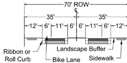
FIGURE 5-3.12 MINOR COLLECTORS -- RURAL/ESL CHARACTER
