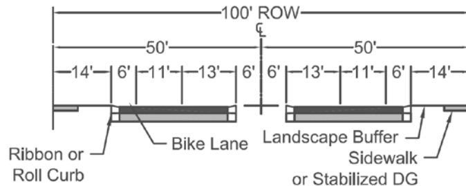
FIGURE 5-3.8 MAJOR COLLECTORS -- RURAL/ESL CHARACTER
