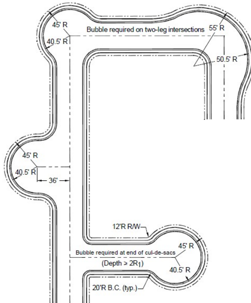
FIGURE 5-3.45 BUBBLES FOR STREETS
