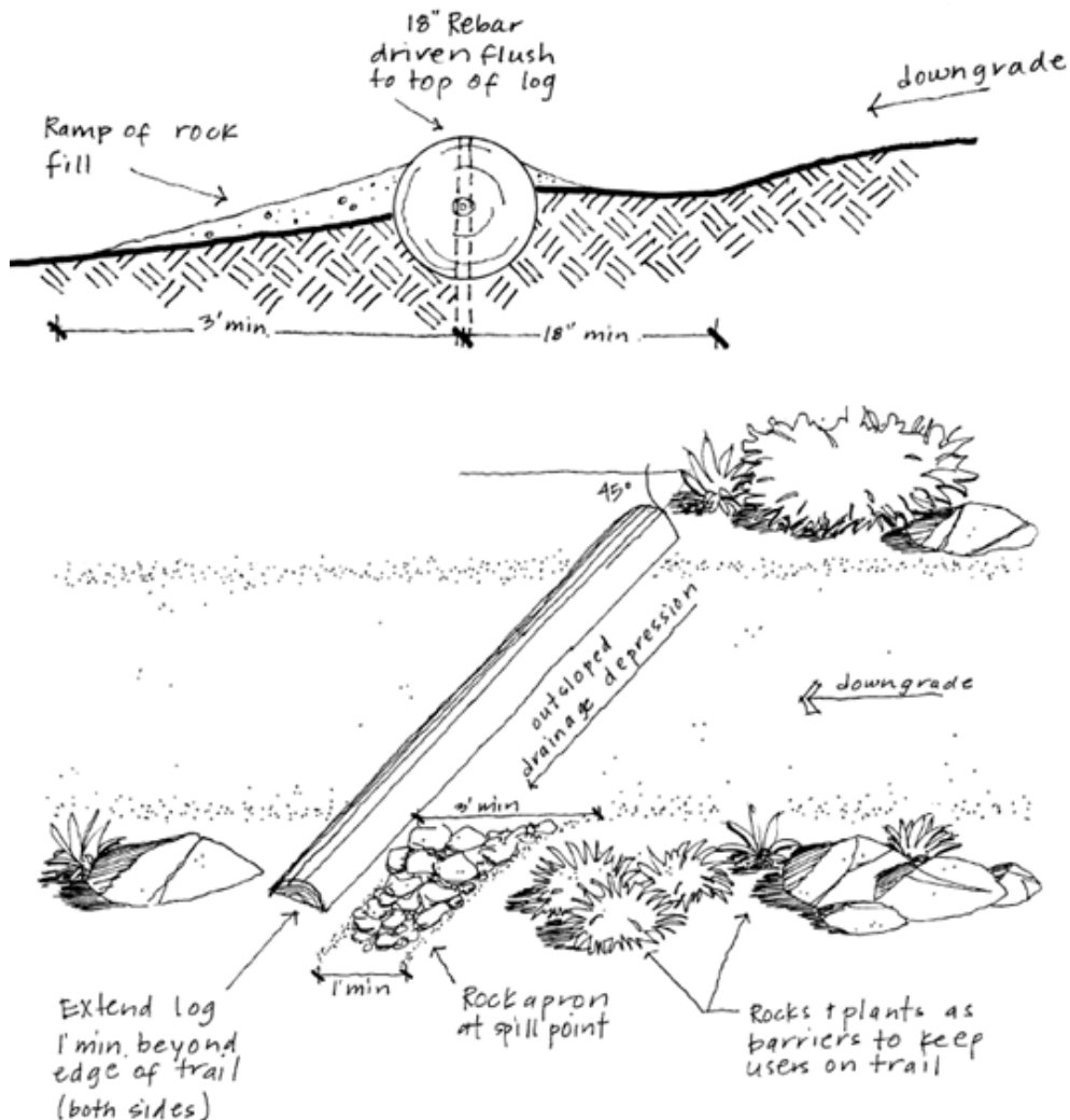
FIGURE 8-3.7 LOG WATERBAR
