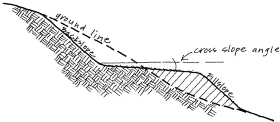
FIGURE 8-3.2 TYPICAL TRAIL PROFILE
