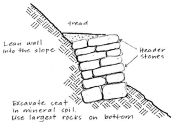
FIGURE 8-3.10 ROCK RETAINING WALLS
