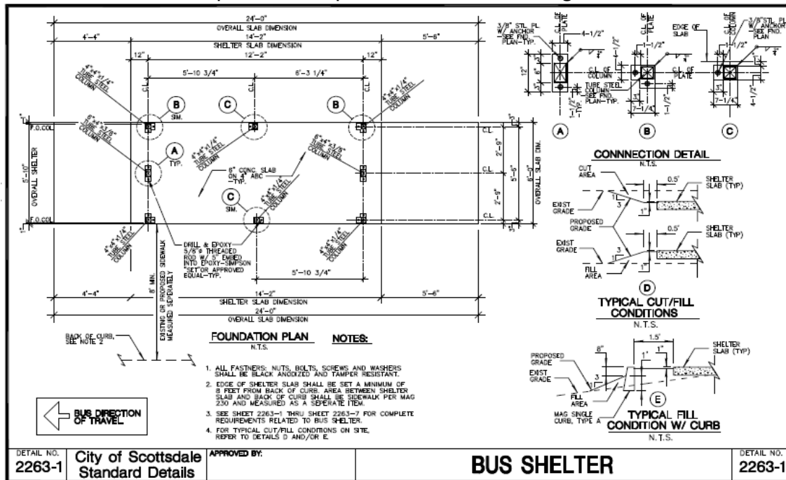
FIGURE 5-6.7 BUS SHELTER FOUNDATION PLAN
