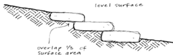
FIGURE 8-3.16 ROCK STEPS
