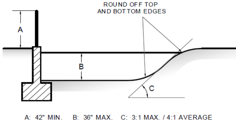
FIGURE 2-1.9 DETENTION BASINS
