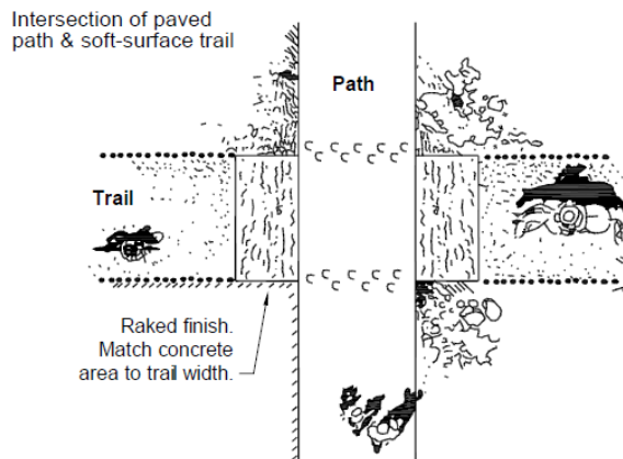
FIGURE 5-7.7 PATH – PATH INTERSECTIONS
