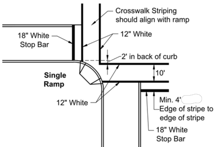
FIGURE 5-5.14 SINGLE RAMP CROSSWALK MARKINGS
