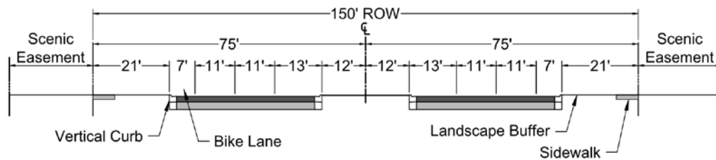
FIGURE 5-3.2 MAJOR ARTERIALS -- SUBURBAN CHARACTER
