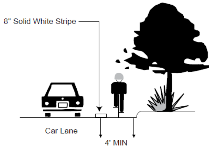
FIGURE 5-7.1 BIKE LANE WHERE PARKING IS PROHIBITED
