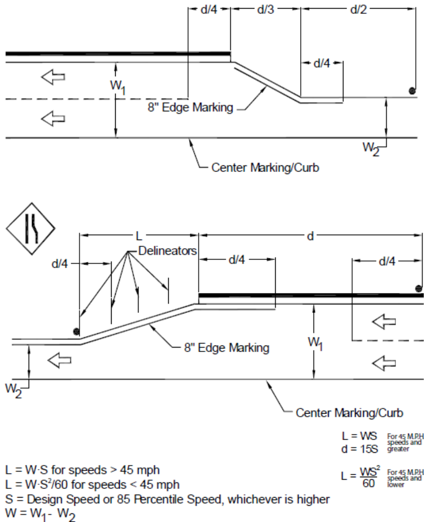
FIGURE 5-3.42 PAVEMENT WIDTH TRANSITIONS
