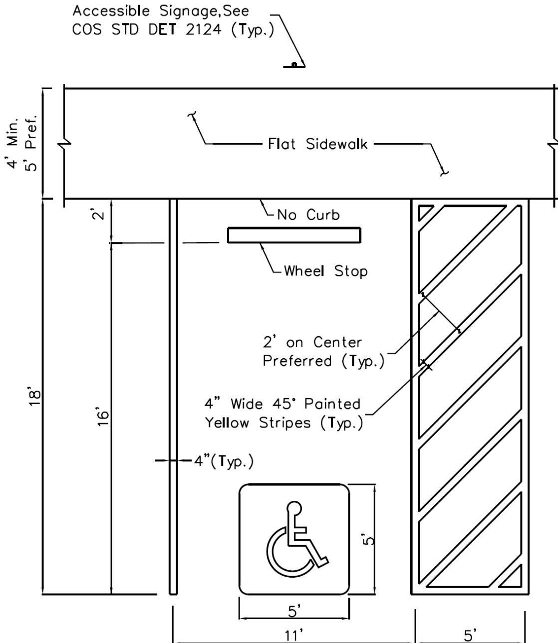
B. SIDEWALK OR PREPARED WALKWAY AT SAME LEVEL AS PARKING
