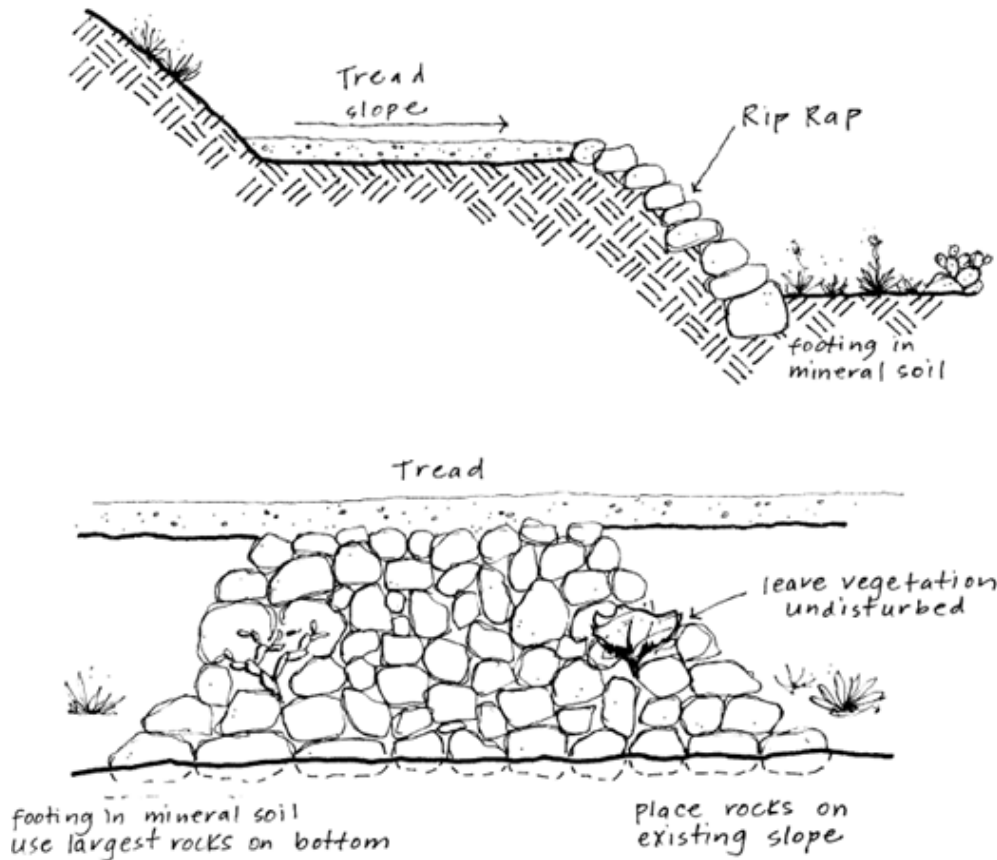
FIGURE 8-3.11 RIPRAP
