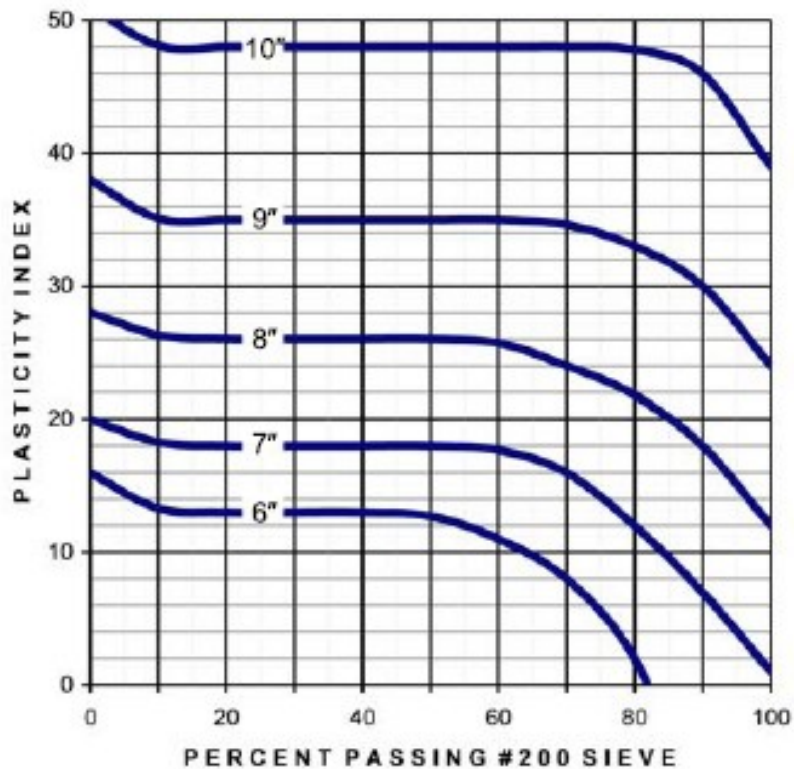
FIGURE 5-10.2 MINIMUM DEPTH OF BASE COURSE FOR LOCAL RESIDENTIAL STREETS
