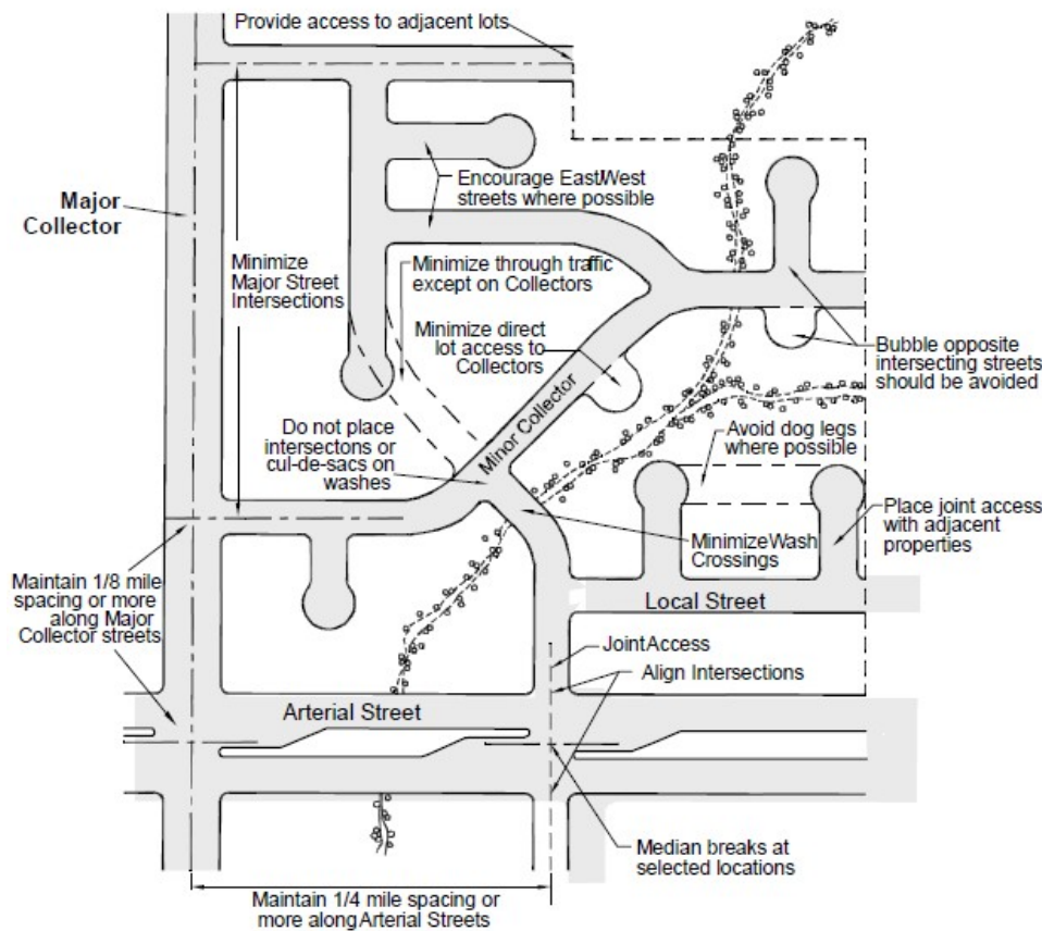
FIGURE 5-3.43 SUBDIVISION STREET PLANNING
