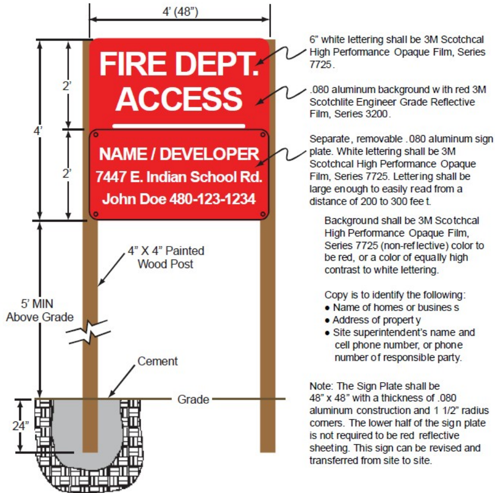
FIGURE 11-1.1 CONSTRUCTION ACCESS SIGN
