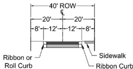
FIGURE 5-3.19 LOCAL RESIDENTIAL -- RURAL/ESL CHARACTER
