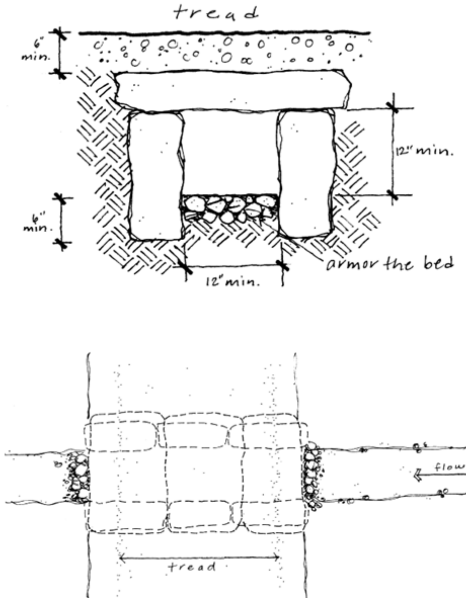
FIGURE 8-3.8 ROCK CULVERT
