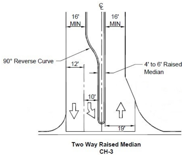
FIGURE 5-3.39 TYPE CH TWO-WAY DRIVEWAYS WITH RAISED MEDIAN
