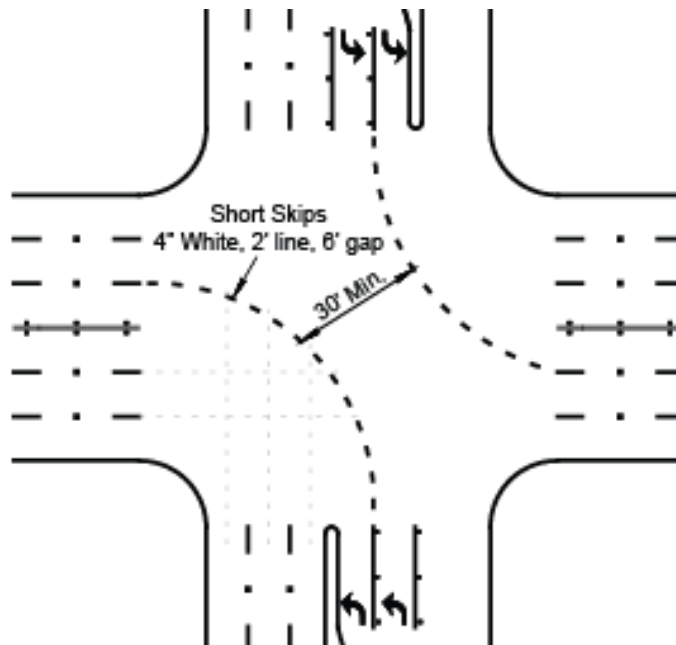
FIGURE 5-5.16 DUAL LEFT TURN INTERSECTION
