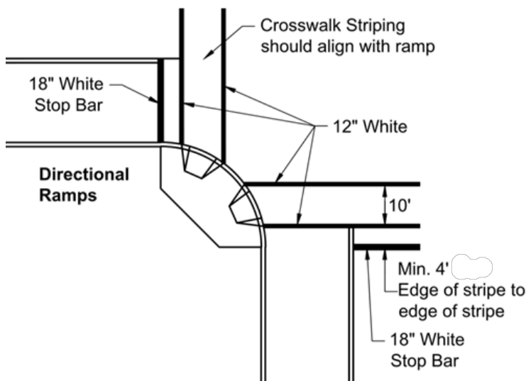
FIGURE 5-5.15 DIRECTIONAL RAMP CROSSWALK MARKINGS
