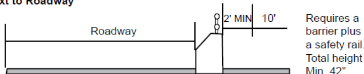
FIGURE 5-7.5 SHARED-USE OR MULTIUSE PATH PERSPECTIVES
