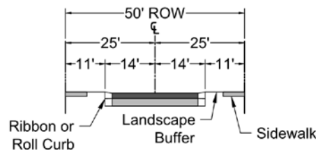
FIGURE 5-3.16 LOCAL COLLECTORS -- RURAL/ESL CHARACTER
