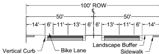
FIGURE 5-3.9 MAJOR COLLECTORS -- SUBURBAN CHARACTER
