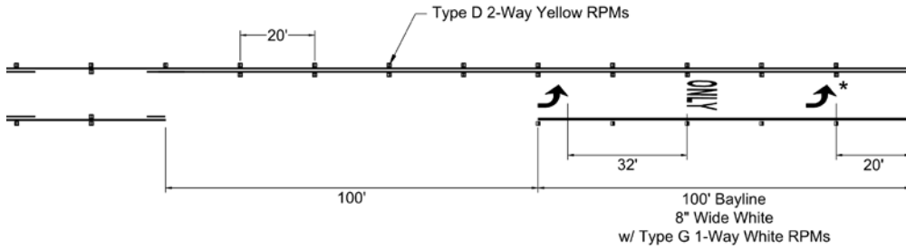
FIGURE 5-5.7 LEFT TURN BAY MARKINGS
