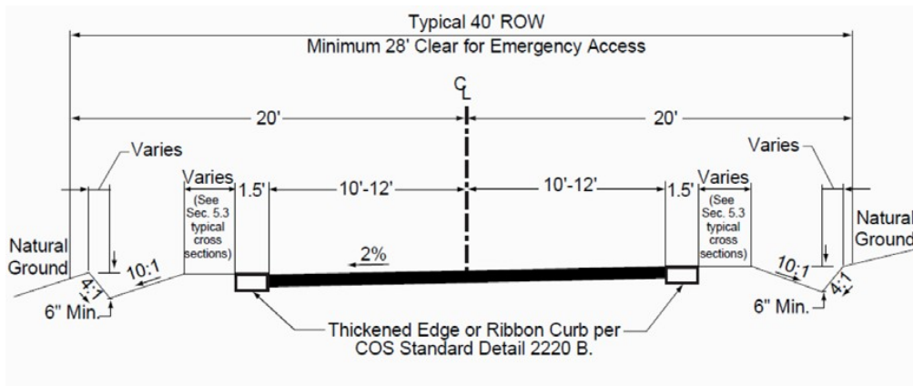
FIGURE 4-1.3 TYPICAL CROSS SECTION FOR ROADSIDE SWALES
