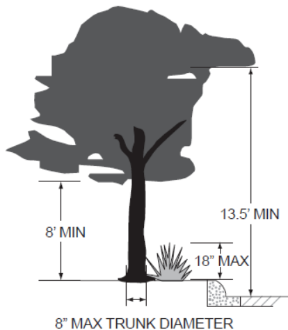
FIGURE 2-1.10 LANDSCAPING IN THE SIGHT VISIBILITY TRIANGLE
