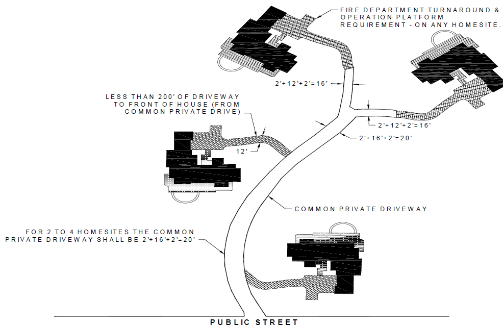
FIGURE 2-2.4 PRIVATE DRIVEWAY DESIGN FOR EMERGENCY ACCESS
