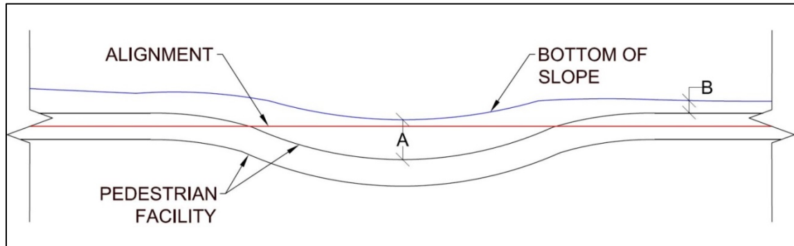
FIGURE 5-3C1: HORIZONTAL CURVE IN PEDESTRIAN FACILITY
