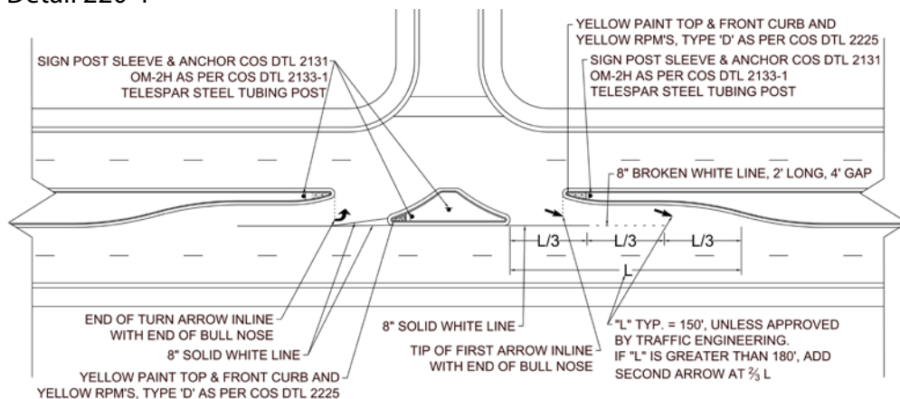
FIGURE 5-5.9 LEFT-IN/LEFT-OUT MARKINGS AND SIGNING
