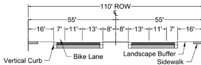
FIGURE 5-3.5 MINOR ARTERIALS -- SUBURBAN CHARACTER
