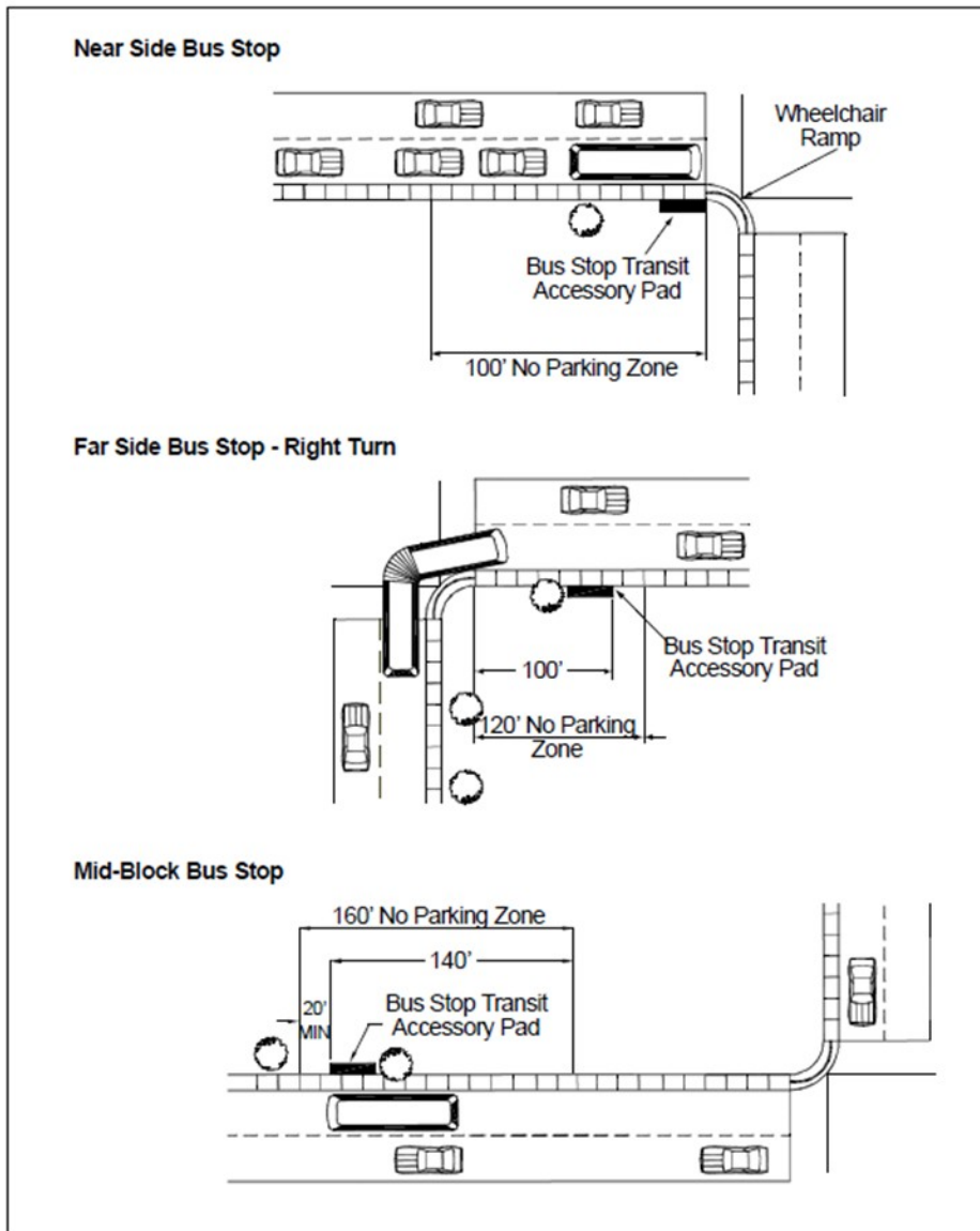
FIGURE 5-6.2 SPECIAL CONDITIONS BUS STOP LOCATIONS
