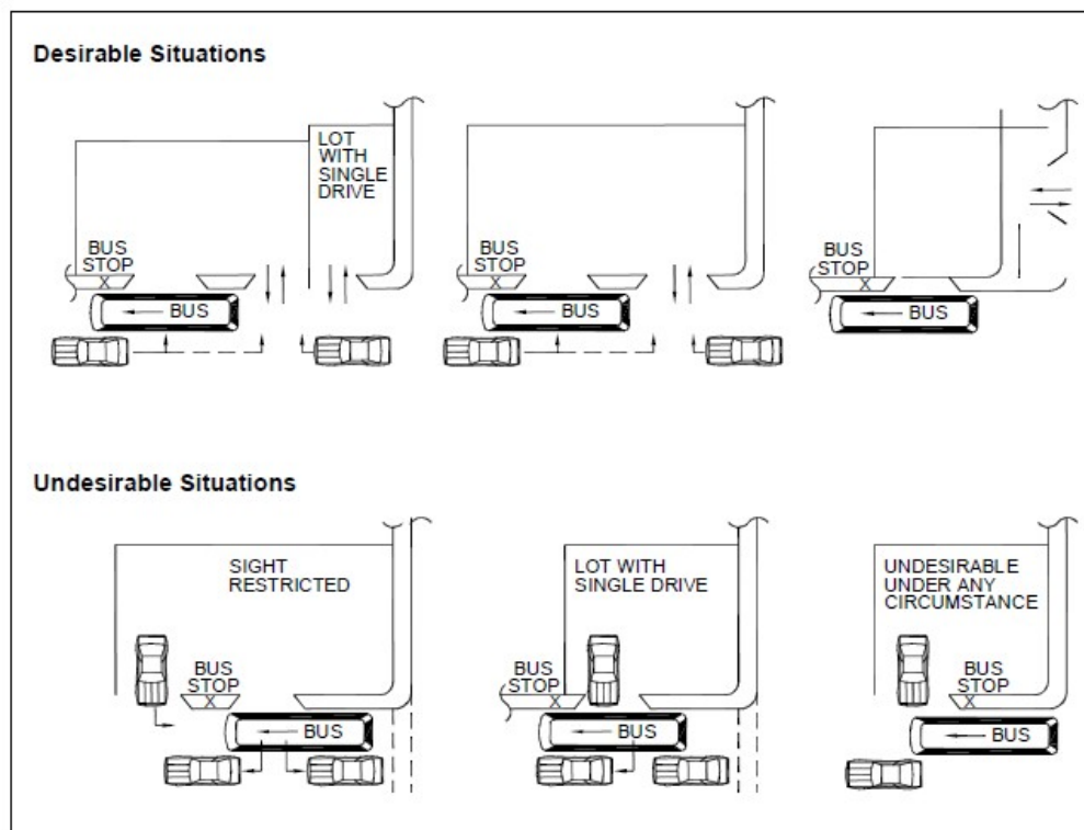
FIGURE 5-6.3 DRIVEWAY LOCATIONS NEAR BUS STOP
