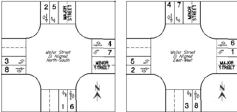
FIGURE 5-4A1 NEMA STANDARD MOVEMENTS
