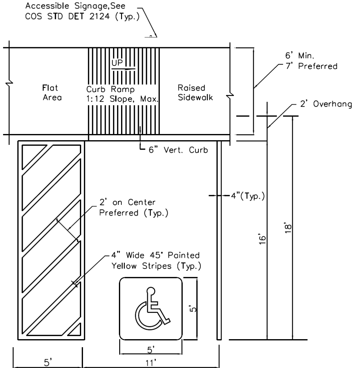
A. SIDEWALK OR PREPARED WALKWAY AS RAISED SIDEWALK FIGURE 12-1.1 PREFERRED ACCESSIBLE PARKING SPACES
