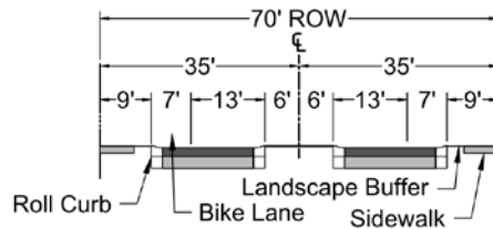
FIGURE 5-3.13 MINOR COLLECTORS -- SUBURBAN CHARACTER
