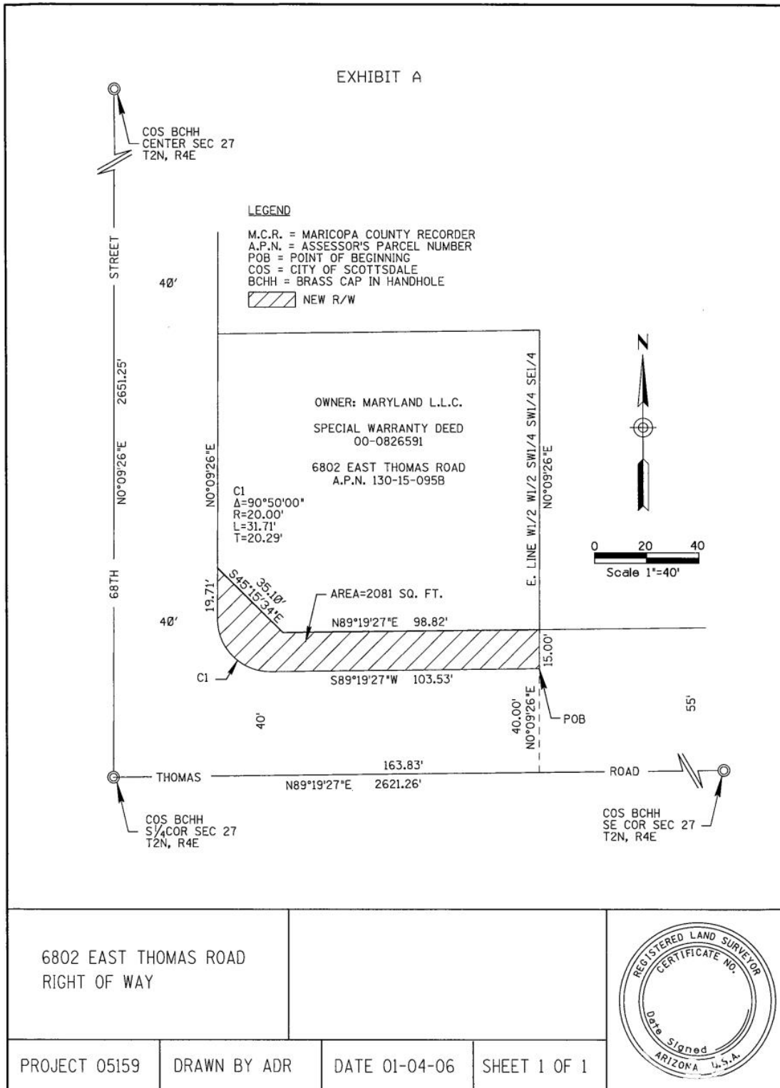
FIGURE 9-1.10 SAMPLE ROW PARCEL EXHIBIT
