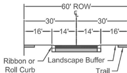
FIGURE 5-3.15 LOCAL COLLECTORS -- RURAL/ESL WITH TRAILS
