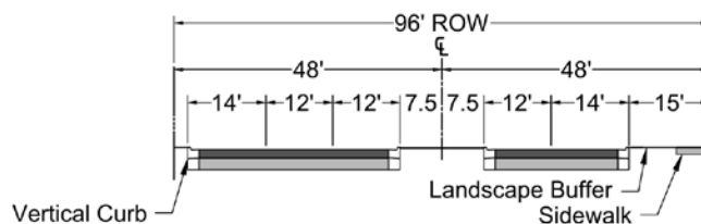
FIGURE 5-3.7 COUPLET STREETS
