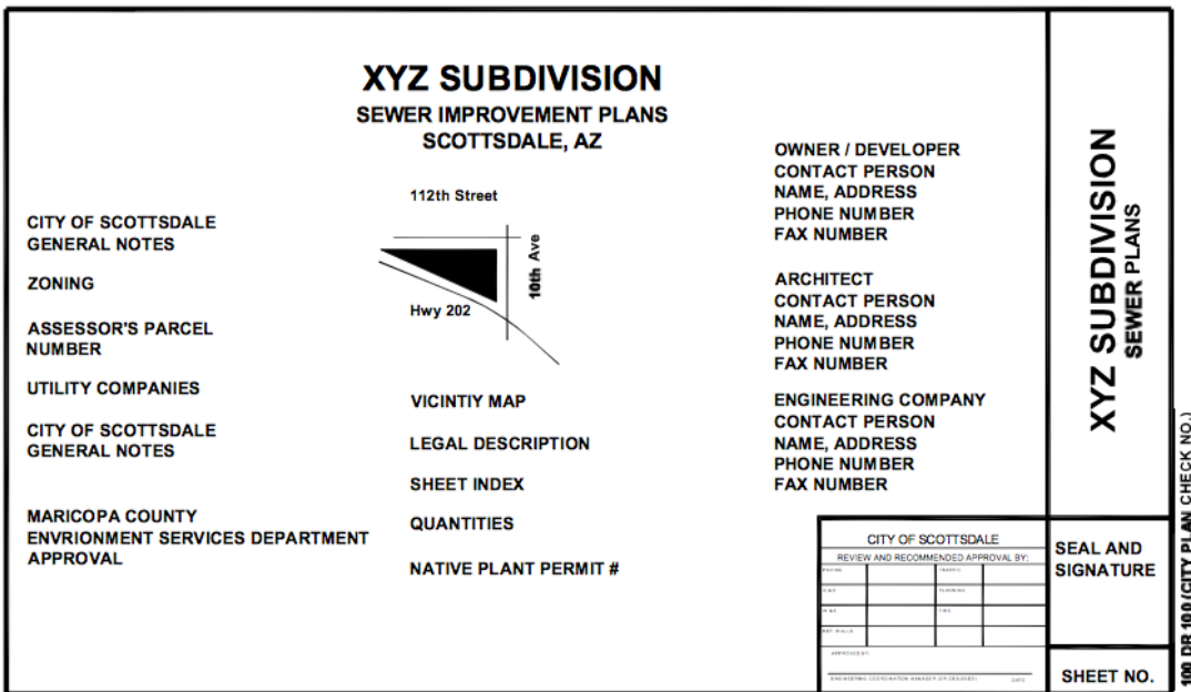
FIGURE 1-3.1 TYPICAL COVER SHEET
