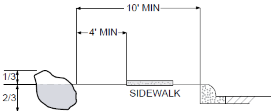
FIGURE 2-1.12 BOULDER PLACEMENTS
