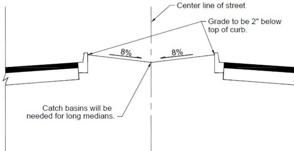
FIGURE 5-3.23 MEDIAN GRADING300
