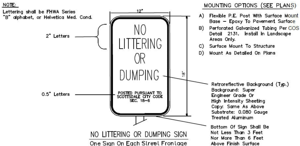
FIGURE 1-2.4 NO LITTERING OR DUMPING SIGN
