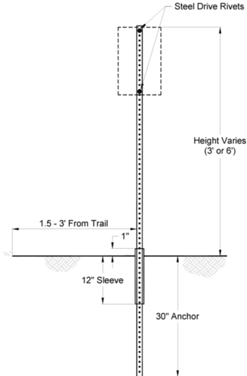
FIGURE 8-3.19 TRAIL SIGN INSTALLATION
