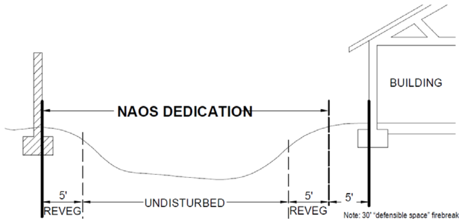
FIGURE 2-2.9 NAOS LOCATION GUIDE
