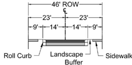
FIGURE 5-3.20 LOCAL RESIDENTIAL -- SUBURBAN CHARACTER
