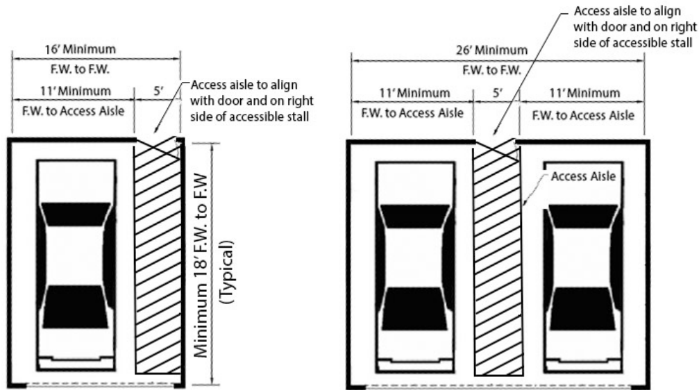
A, One Space Adaptable Accessible Parking Garage
