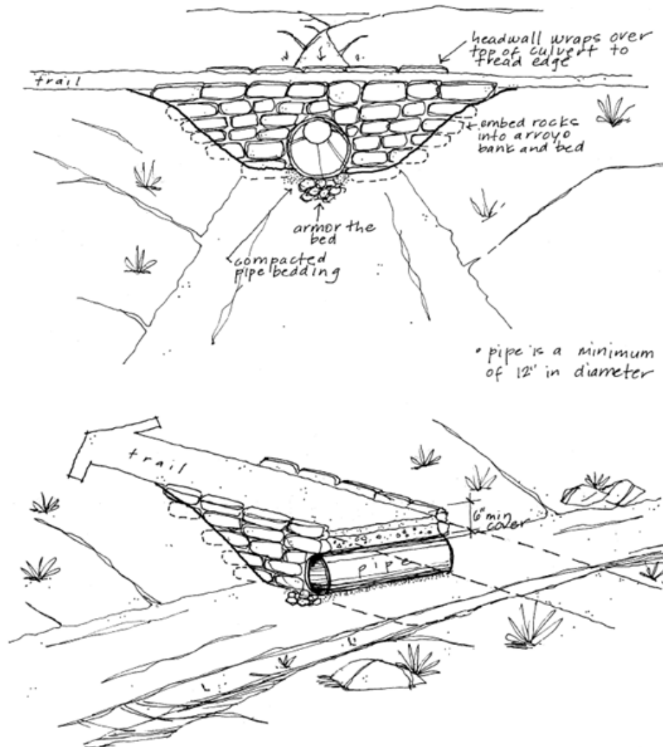
FIGURE 8-3.9 PIPE CULVERT
