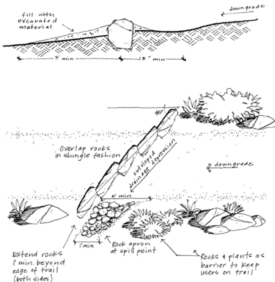
FIGURE 8-3.6 ROCK WATERBAR
