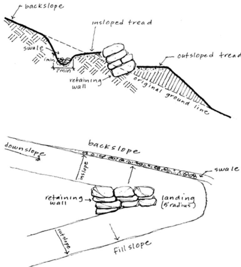
FIGURE 8-3.14 SWITCHBACK TURN
