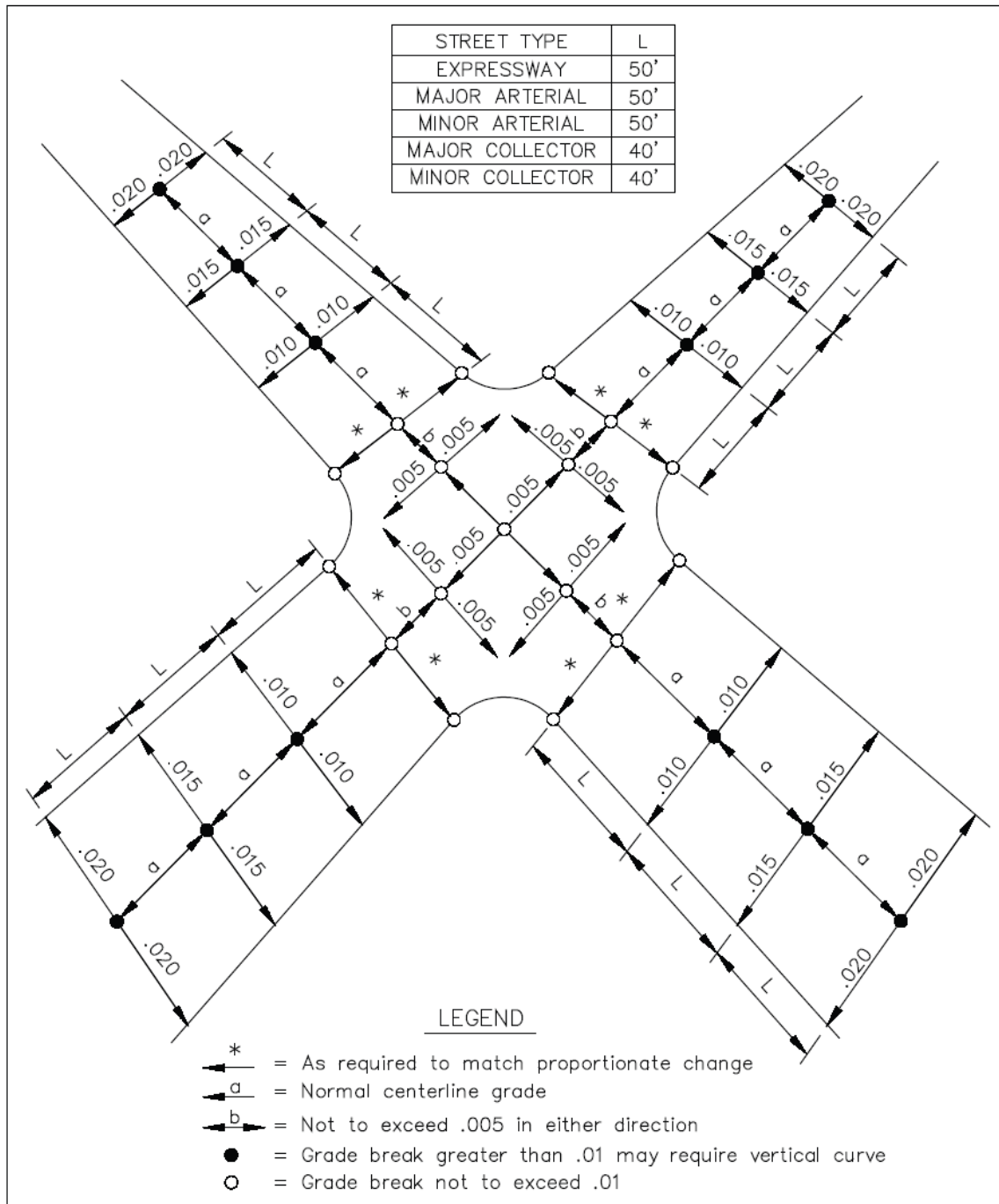
FIGURE 9-1.6 INTERSECTION CROSS-SLOPES AND CROWN RUN-OFF
