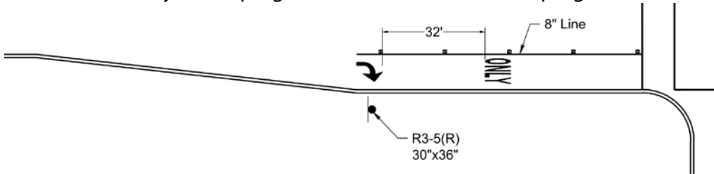
FIGURE 5-5.10 RIGHT TURN BAY MARKINGS
