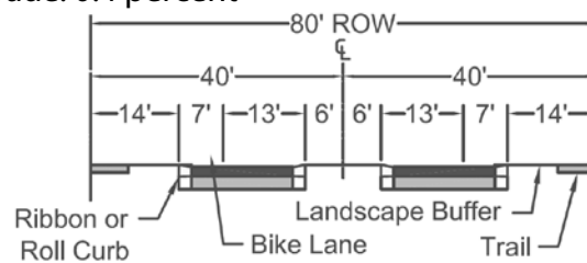
FIGURE 5-3.11 MINOR COLLECTORS -- RURAL/ESL WITH TRAILS
