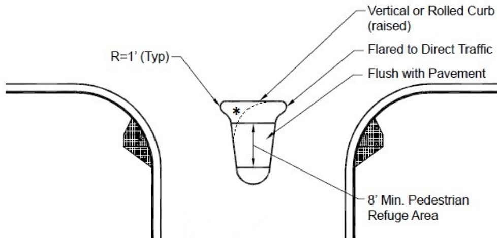
FIGURE 5-3.30 LEFT IN / LEFT IN MEDIAN OPENINGS FOR INTERSECTIONS
