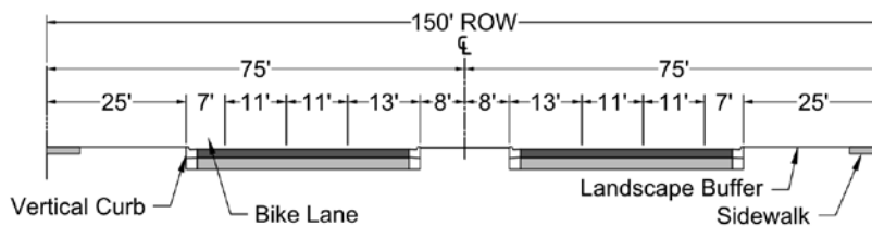
FIGURE 5-3.3 MAJOR ARTERIALS – URBAN CHARACTER
