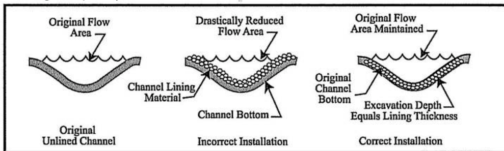
FIGURE 4-1.4 CHANNEL LINING DESIGN CAPACITY
