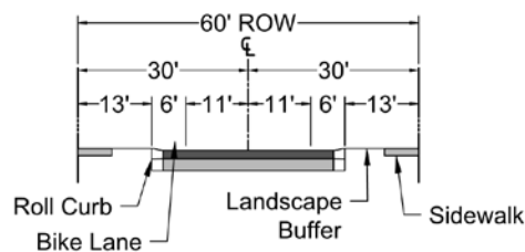
FIGURE 5-3.17 LOCAL COLLECTORS -- SUBURBAN CHARACTER
