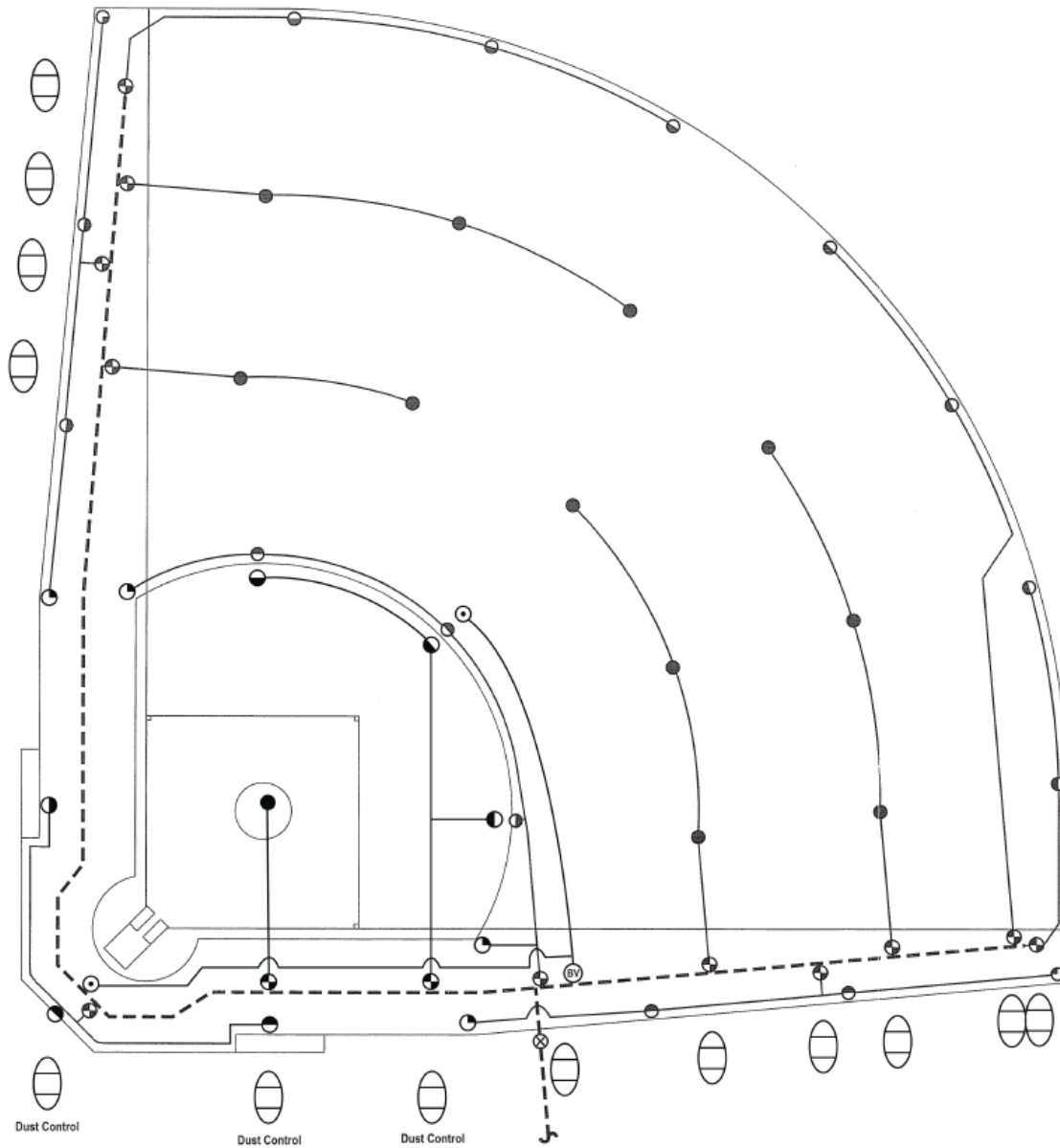
THIS FIGURE IS FOR ILLUSTRATIVE PURPOSES ONLY ALL IRRIGATION HEADS FOR DUST CONTROL ARE TO BE PLACED IN TURF.
