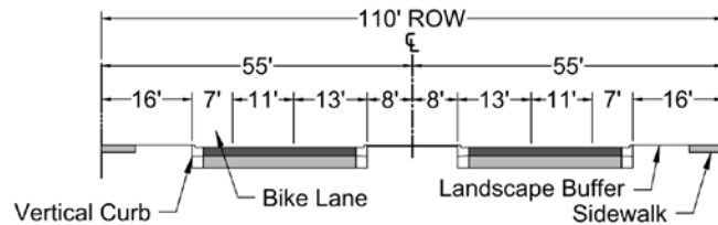
FIGURE 5-3.6 MINOR ARTERIALS -- URBAN CHARACTER
