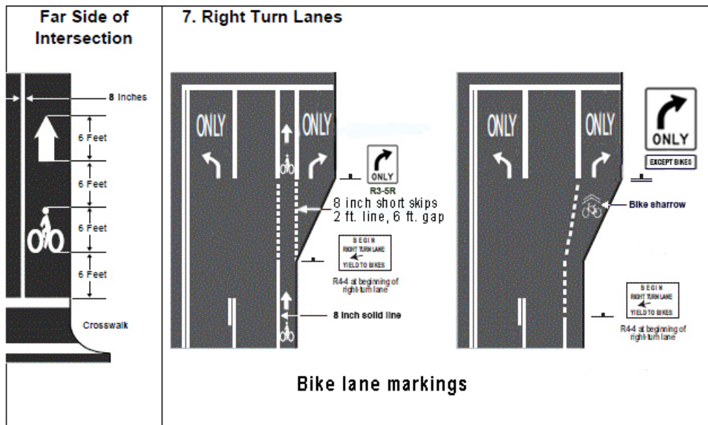
FIGURE 5-5.11 BIKE LANE MARKINGS
