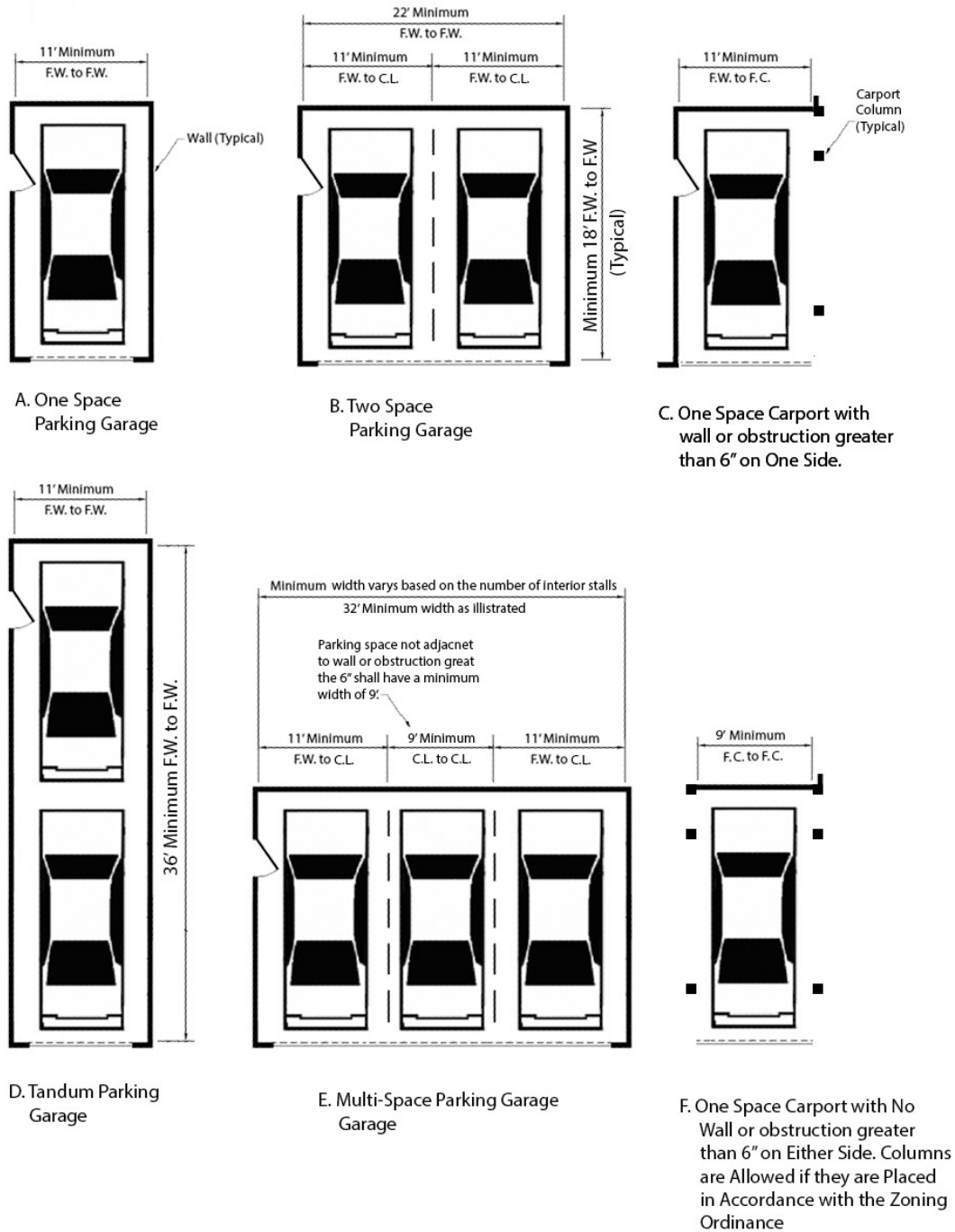
FIGURE 2-1.7 GARAGE AND CARPORT PARKING WIDTH
