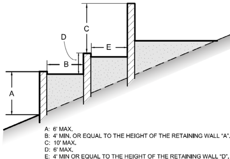
FIGURE 2-2.8 RETAINING WALL DIMENSIONS
