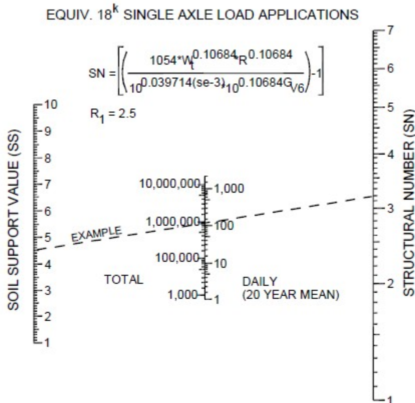
FIGURE 5-10.6 FLEXIBLE PAVEMENTS, 20-YEAR TRAFFIC ANALYSIS
