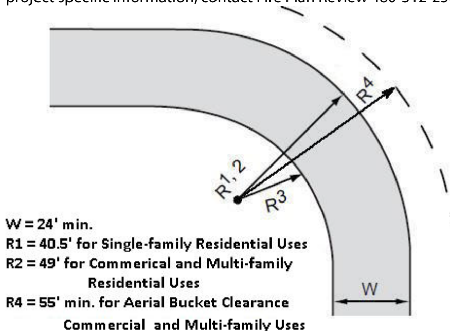
FIGURE 2-1.4 FIRE LANE DIMENSIONS
