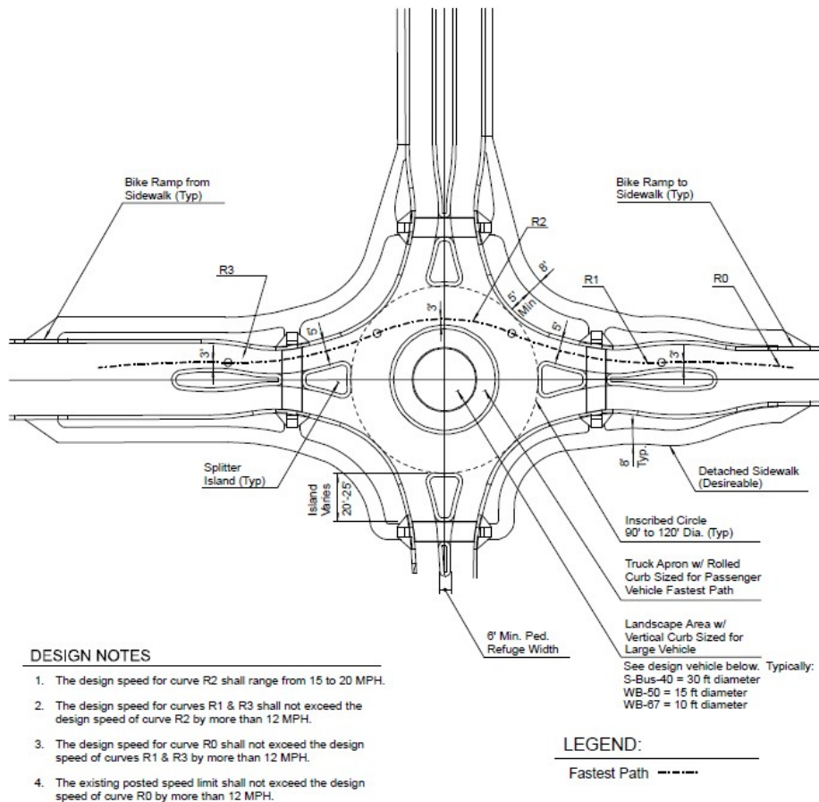
FIGURE 5-3.32 ROUNDABOUT DESIGN
