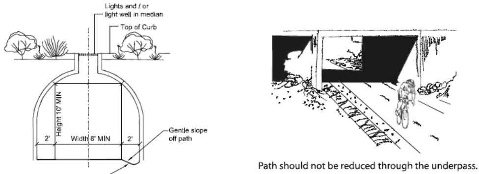
FIGURE 5-7.11 SHARED USE OR MULTIUSE PATH – TUNNELS
