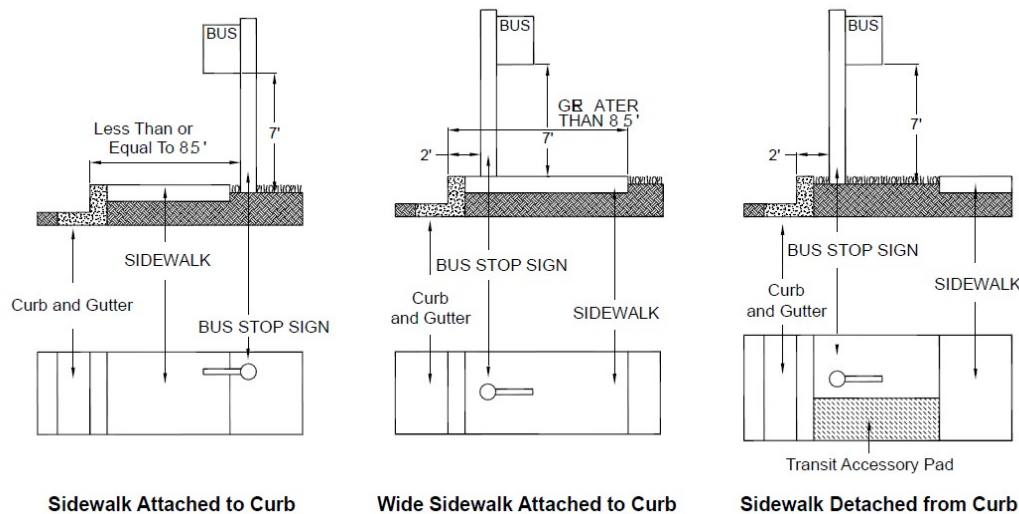
FIGURE 5-6.14 BUS STOP SIGN CLEARANCES
