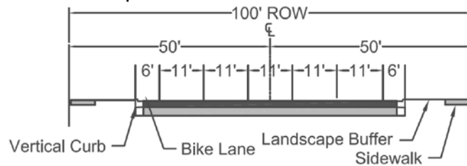
FIGURE 5-3.10 MAJOR COLLECTORS -- URBAN CHARACTER
