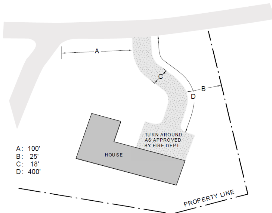
FIGURE 2-2.7 DRIVEWAYS ON HILLSIDE LANDFORM
