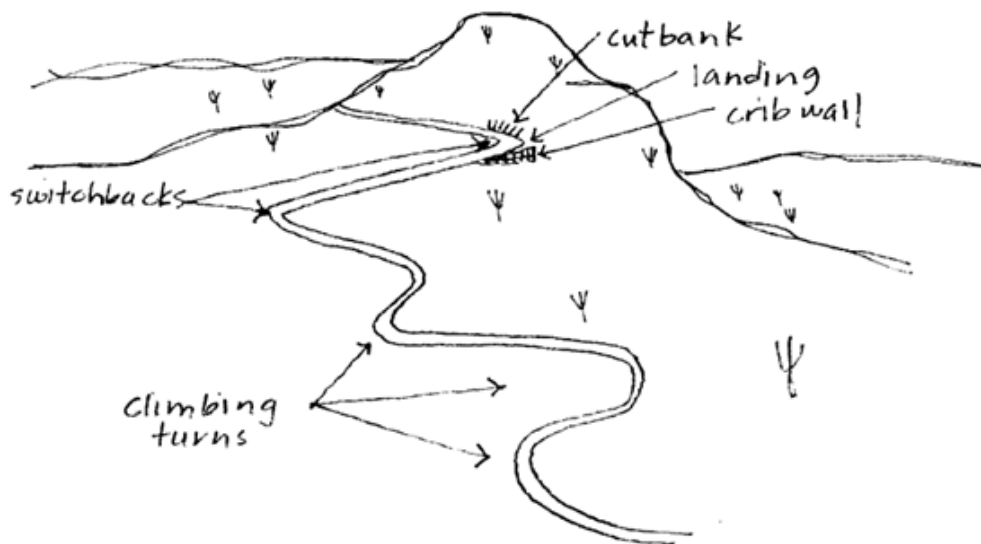
FIGURE 8-3.13 SWITCHBACK AND CLIMBING TURN CONCEPTS
