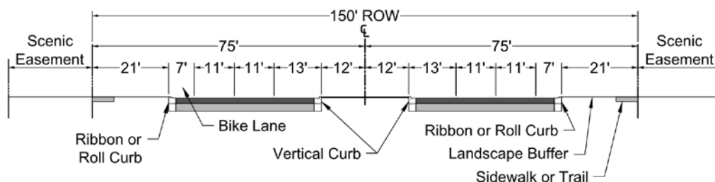
FIGURE 5-3.1 MAJOR ARTERIALS -- RURAL CHARACTER
