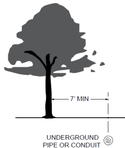
FIGURE 2-1.11 TREE SETBACK FROM UNDERGROUND PIPE OR CONDUIT
