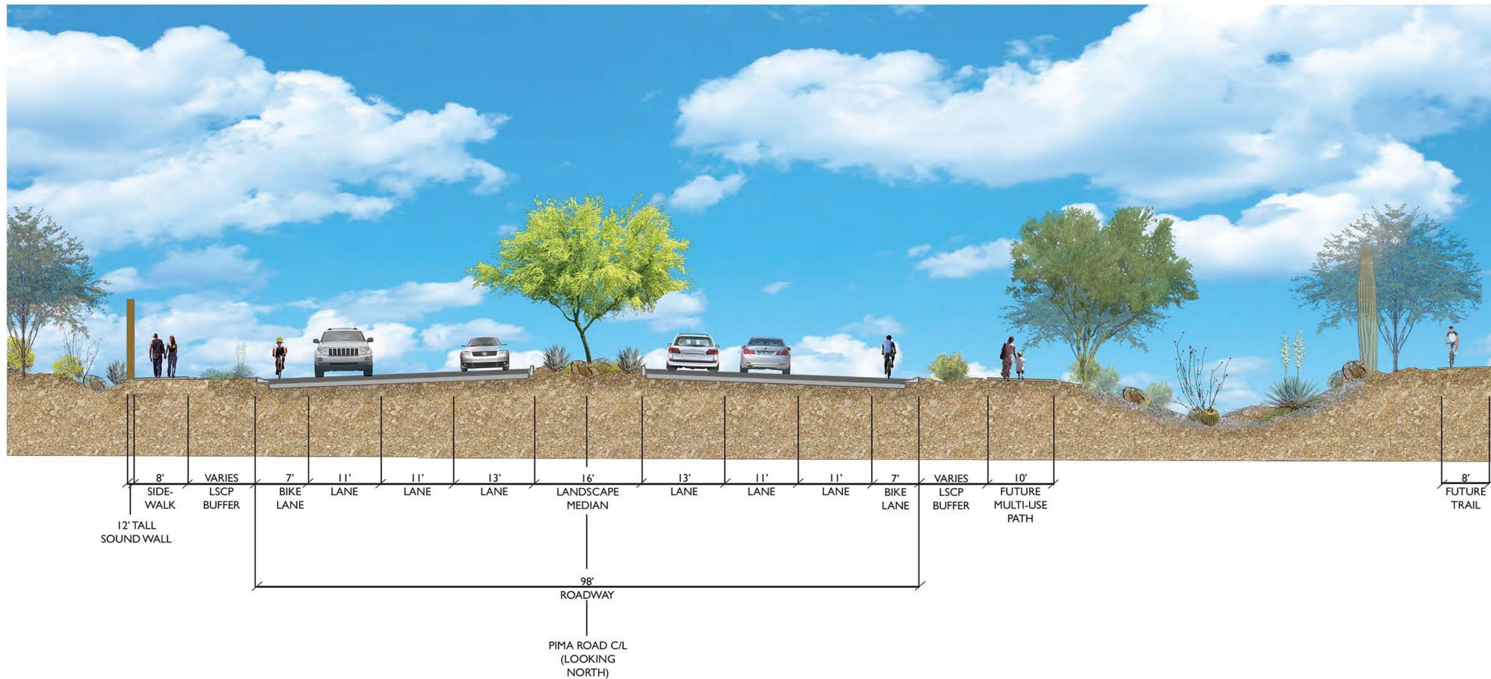
TYPICAL STREET SECTION
