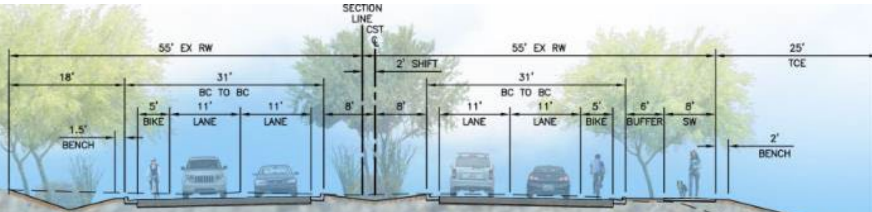
SECTION E-E : STA 202+00 (Looking East)
