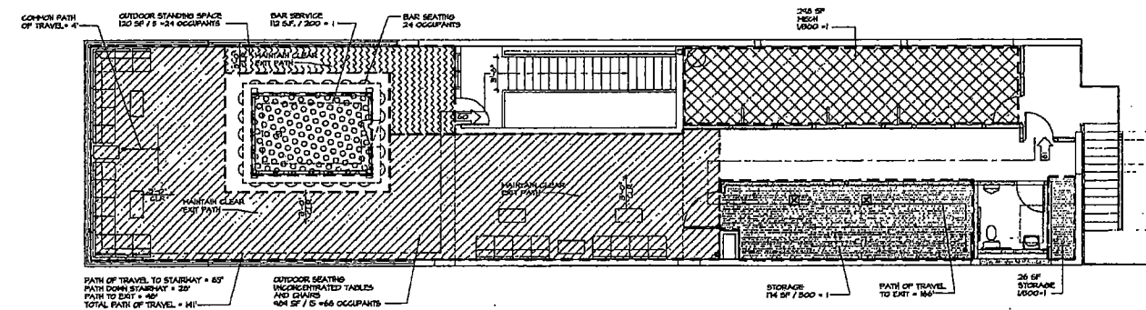
2 SECOND FLOOR EXIT / OCCUPANCY / FURNITURE PLAN SCALE: 3/16" = 1'-0"
