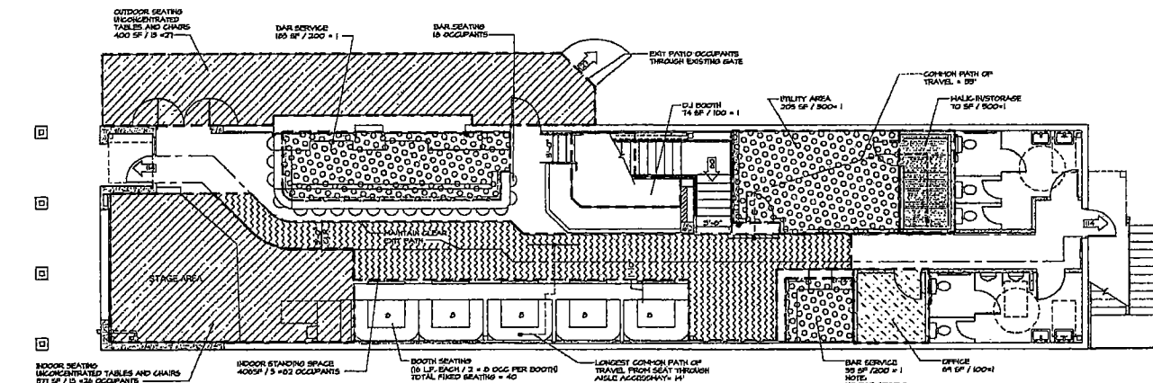
1 FIRST FLOOR EXIT / OCCUPANCY / FURNITURE PLAN SCALE: 3/16" = 1'-0"
