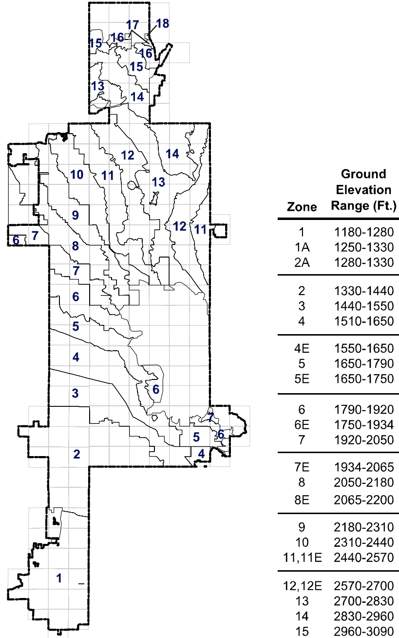
FIGURE 6-3. PRESSURE ZONE MAP
