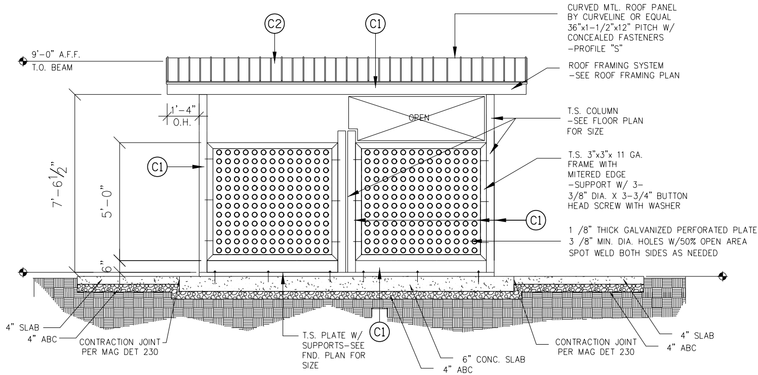
ELEVATION B-B (From 2263-2)
