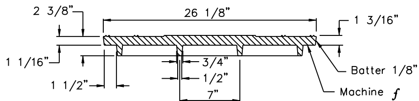
24" MANHOLE COVER
