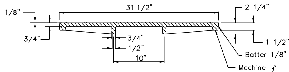
30" MANHOLE COVER
