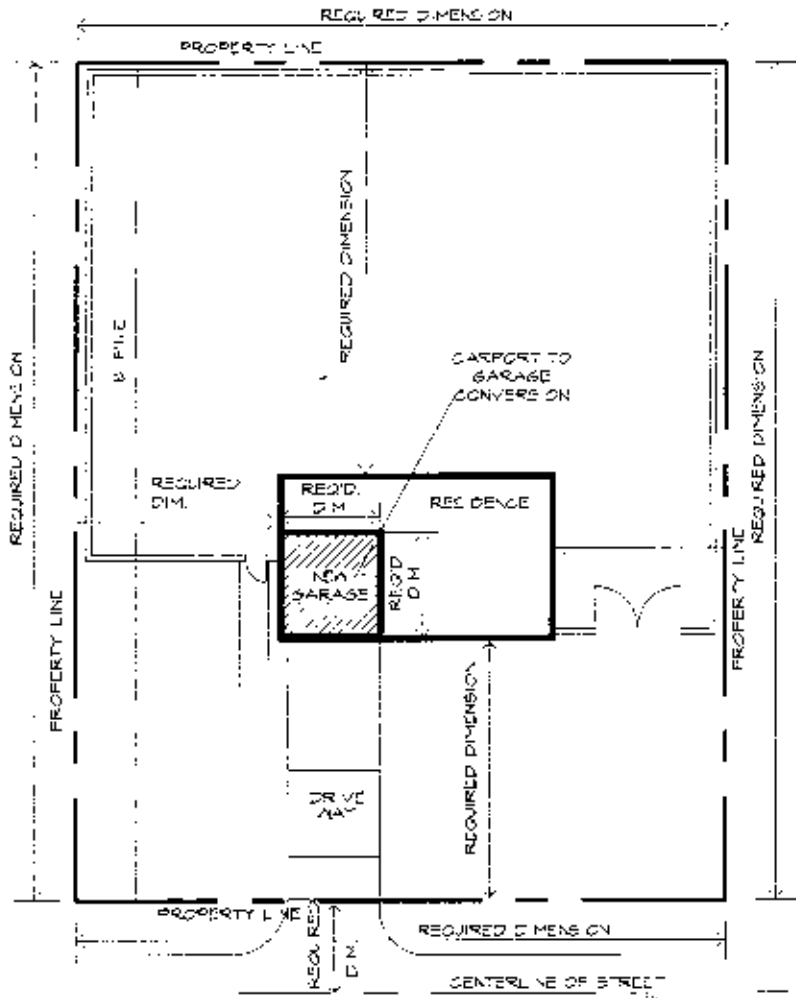
TYPICAL SITE PLAN
