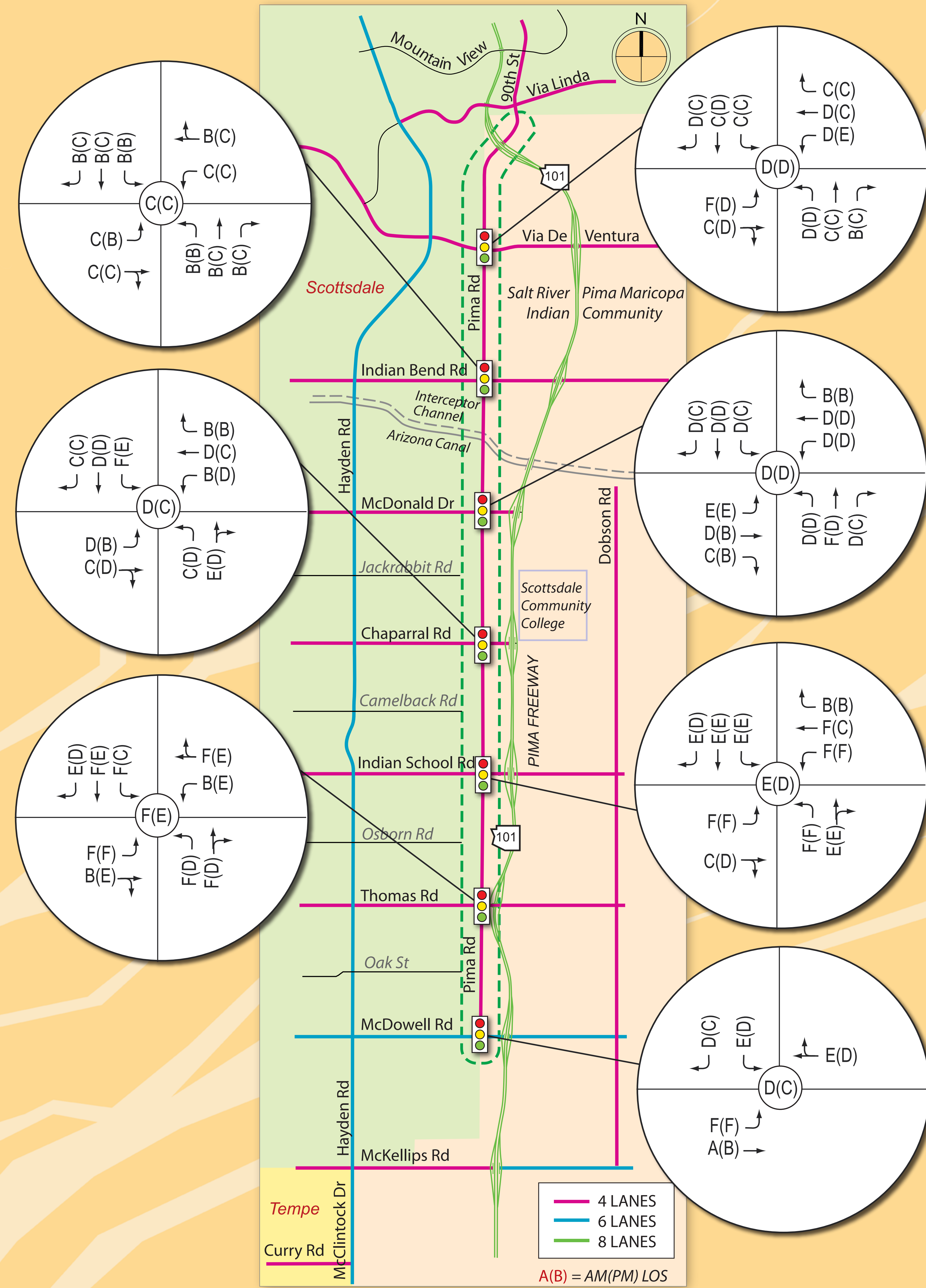
Intersection and Approach Level of Service on Pima Road 2030 Build - 4 Lanes Via DeVentura to McDowell Road
