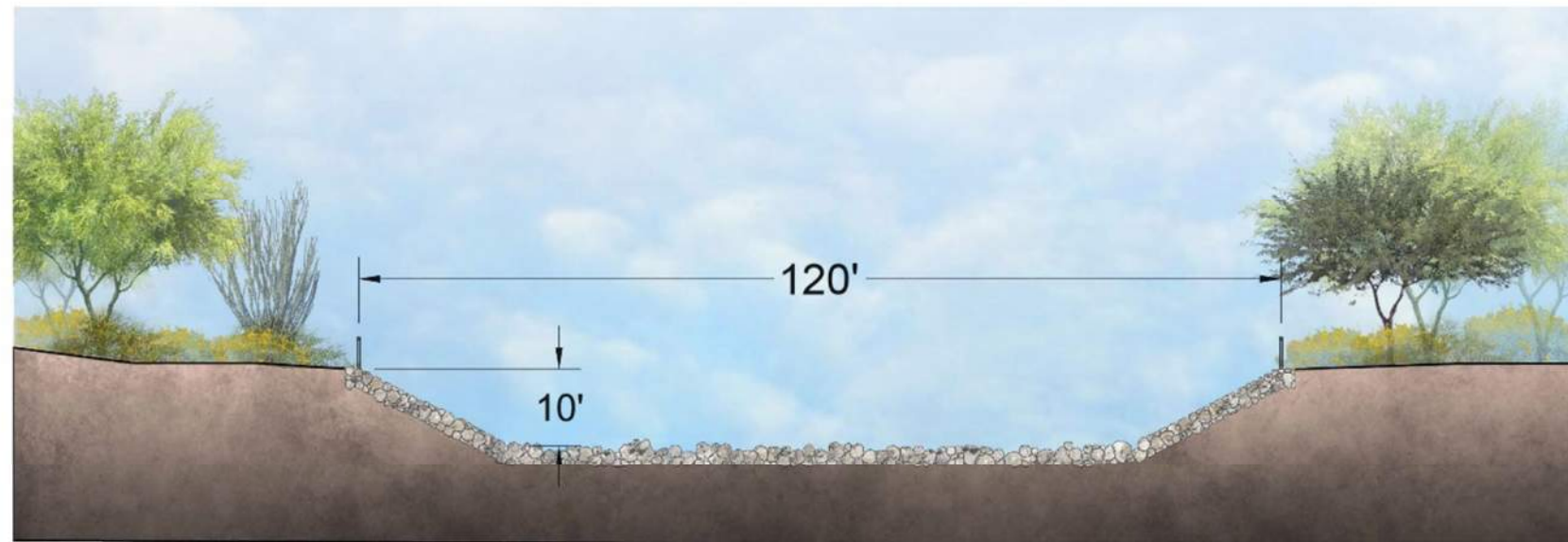
GROUTED ROCK CHANNEL
