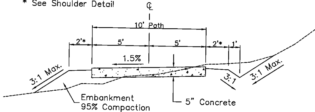
MULTI-USE PATH DETAIL
