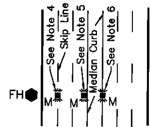
Midblock WITH RAISED MEDIAN
