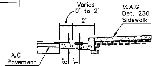
SEC. D-D
