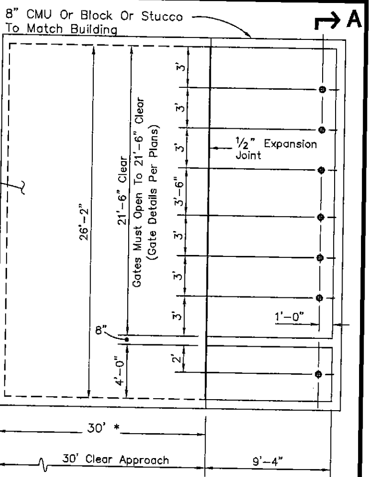
PLAN
