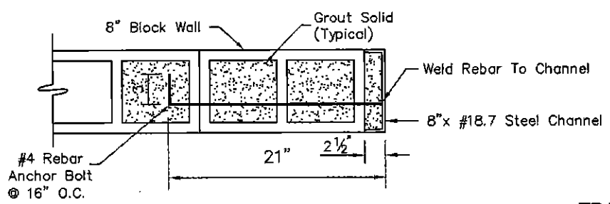
CHANNEL ANCHOR DETAIL
