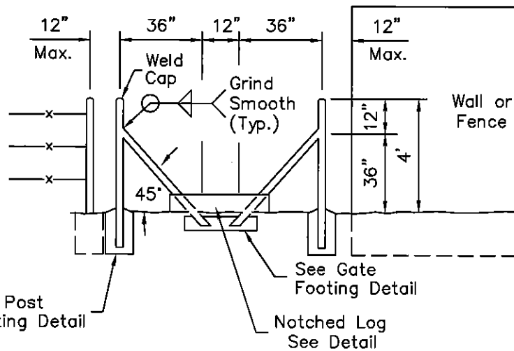
ELEVATION TYPE I GATE
