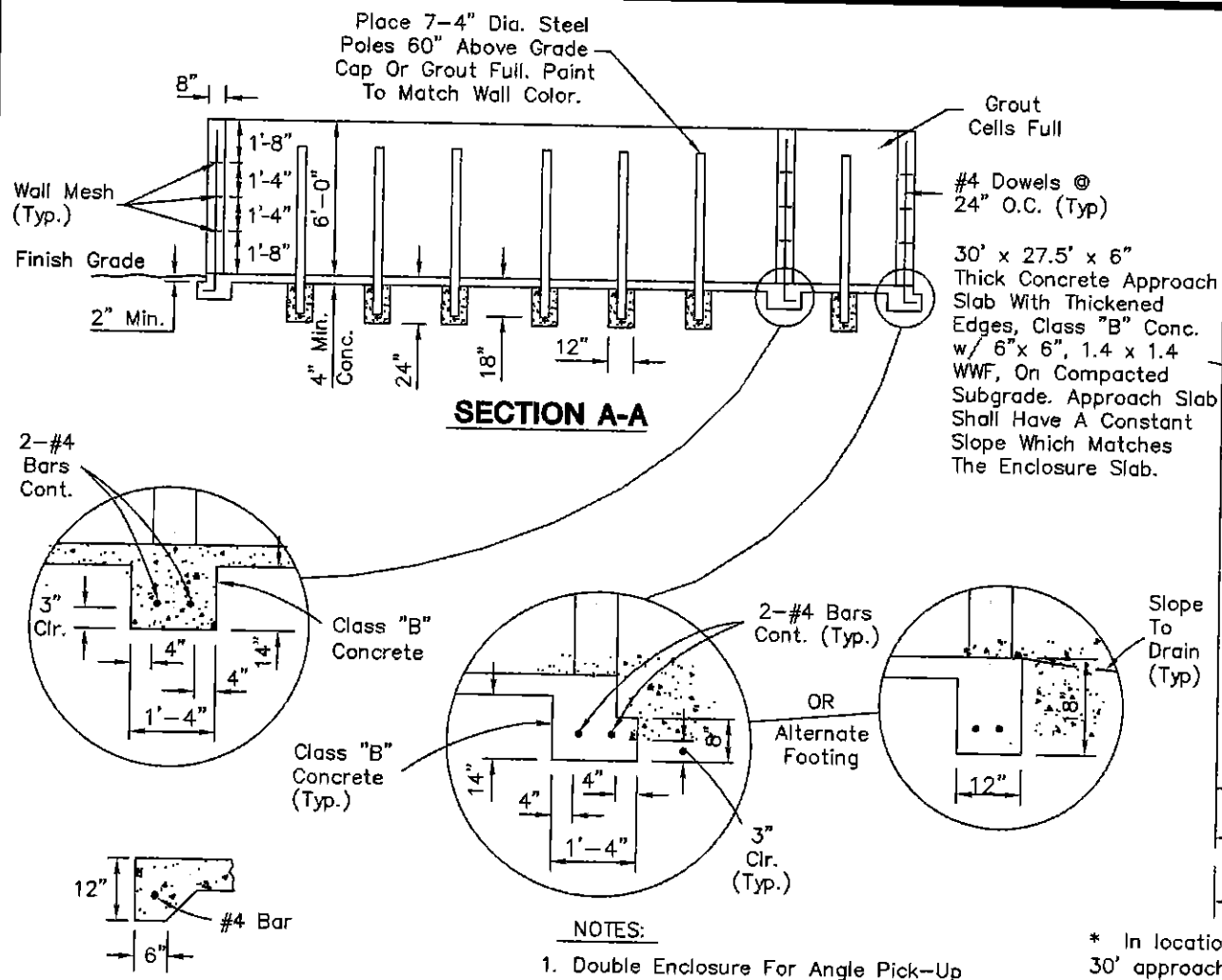
APPROACH SLAB THICKENED EDGE DETAIL
