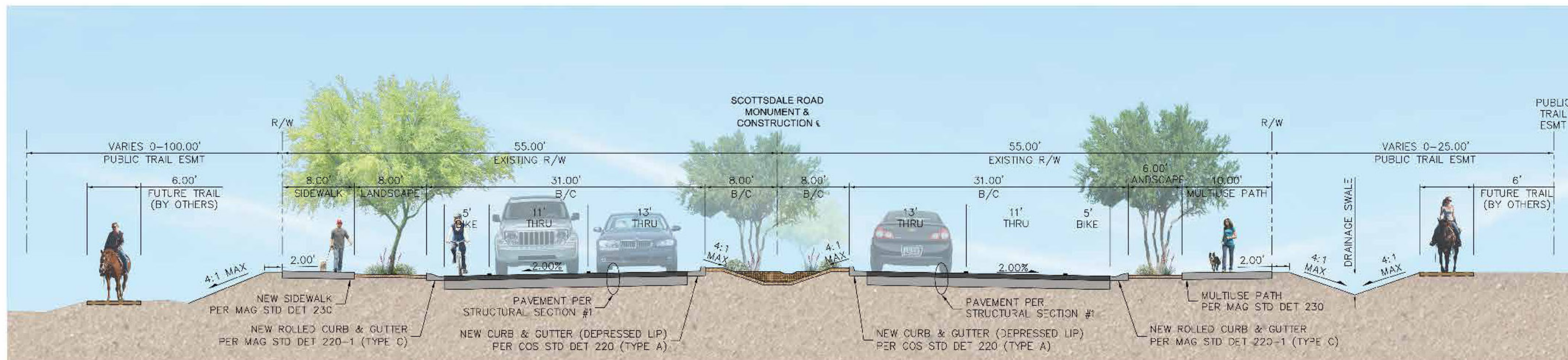
COMPLETE STREETS LANDSCAPE AND LID ELEMENTS "LOOKING NORTH" not to scale
