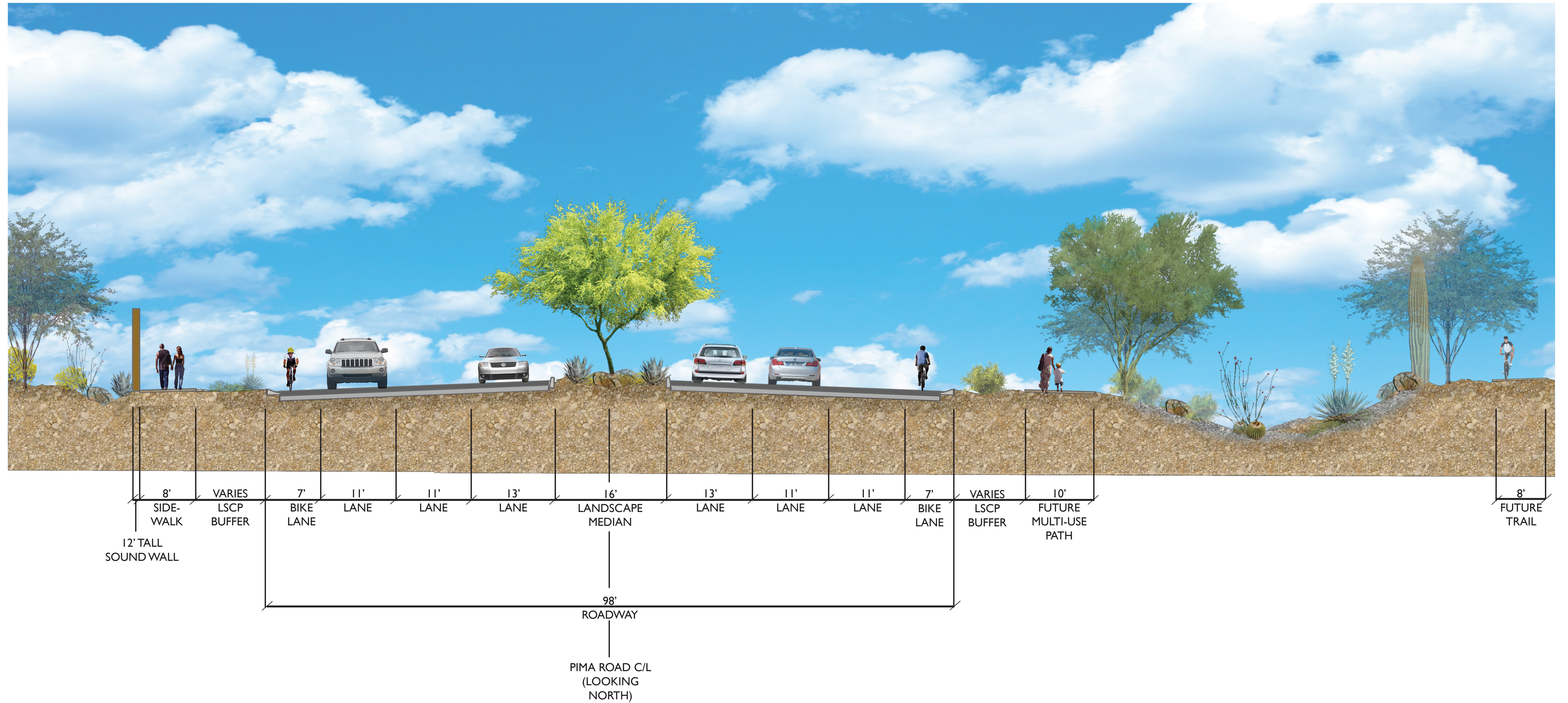
TYPICAL STREET SECTION
